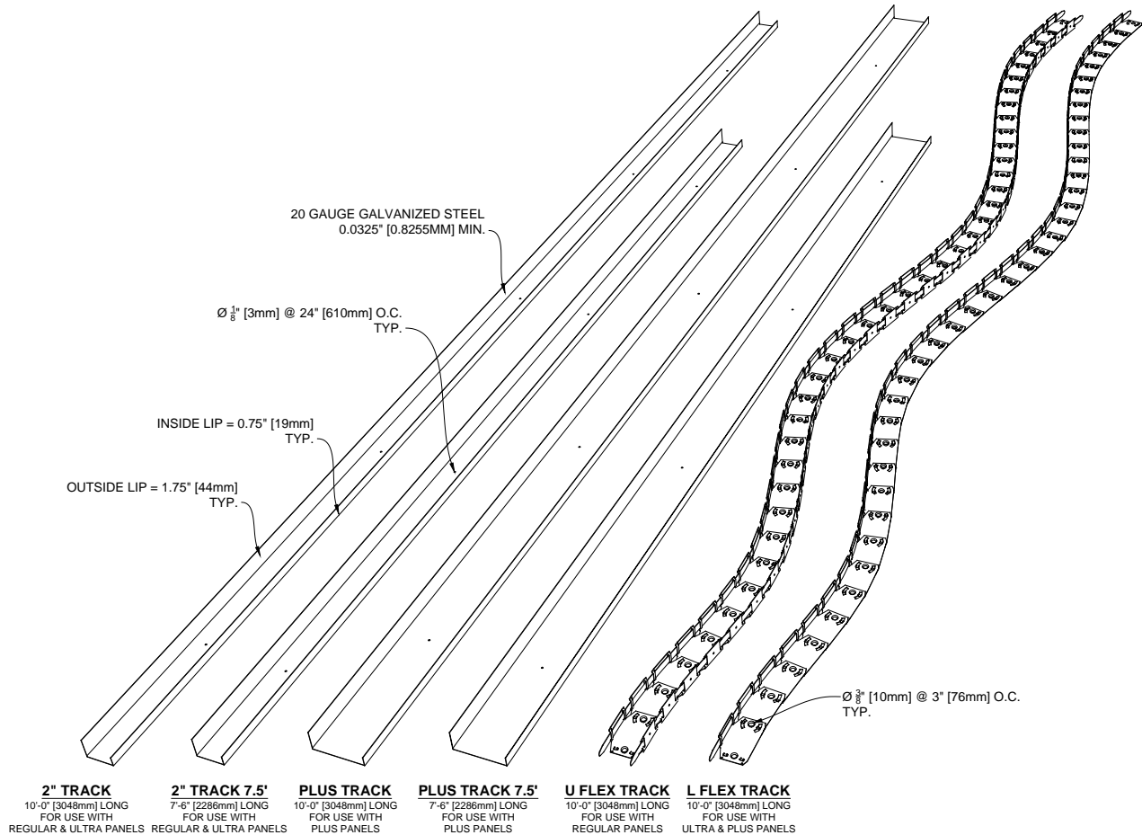
Figure 25: Different Types of Quad-Lock Metal Tracks
