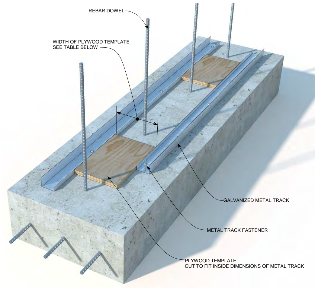
Figure 41: Plywood Templates fit to Wall Dimension
