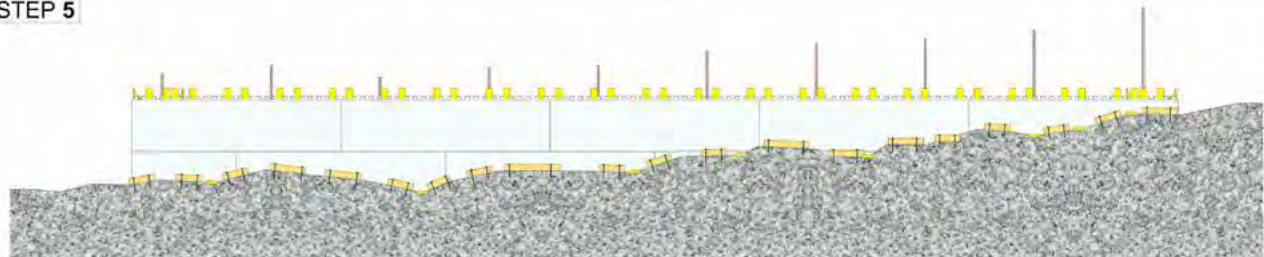
Figure 40: Quad-Lock Wall Installation on Bedrock
