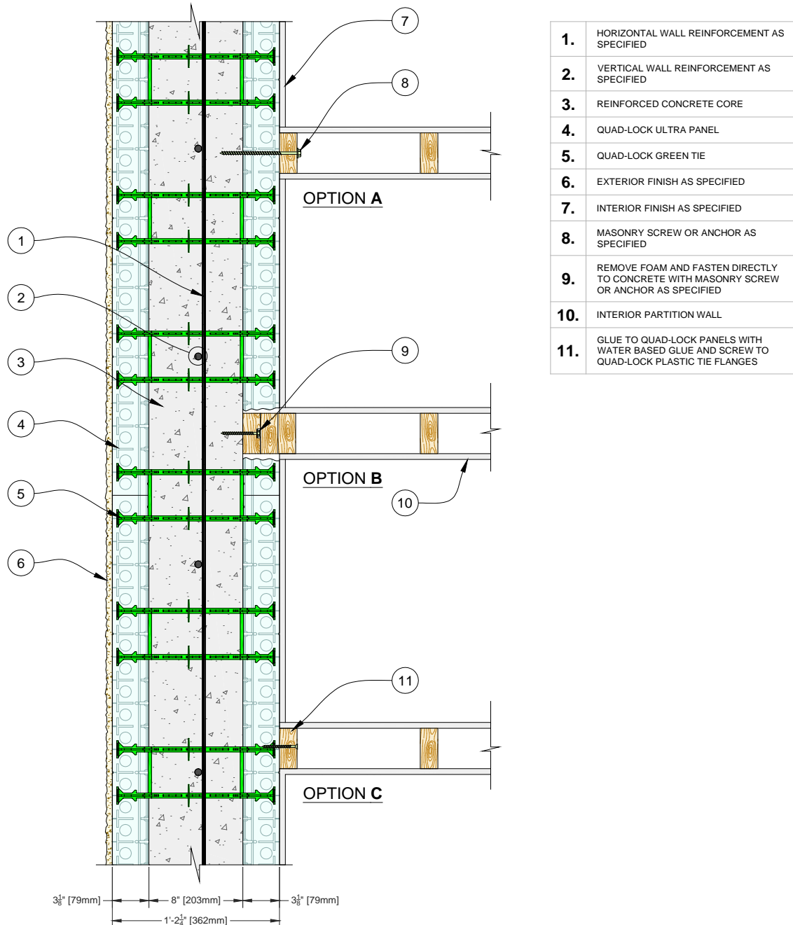
Figure 124: Typical Interior Partition Wall Connections (plan view)
