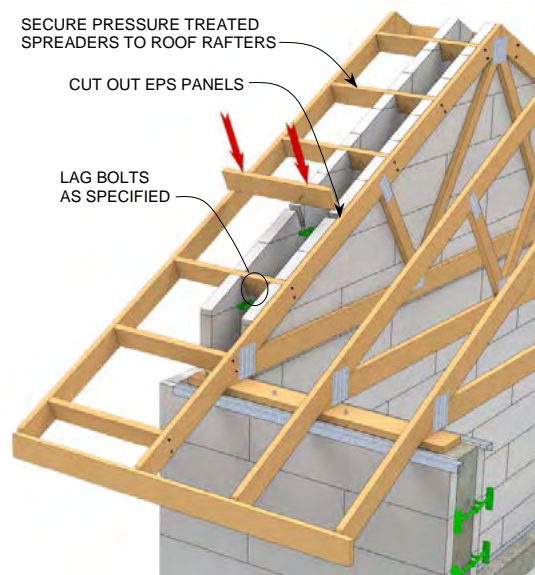
STEP 3 Overhang Installation
