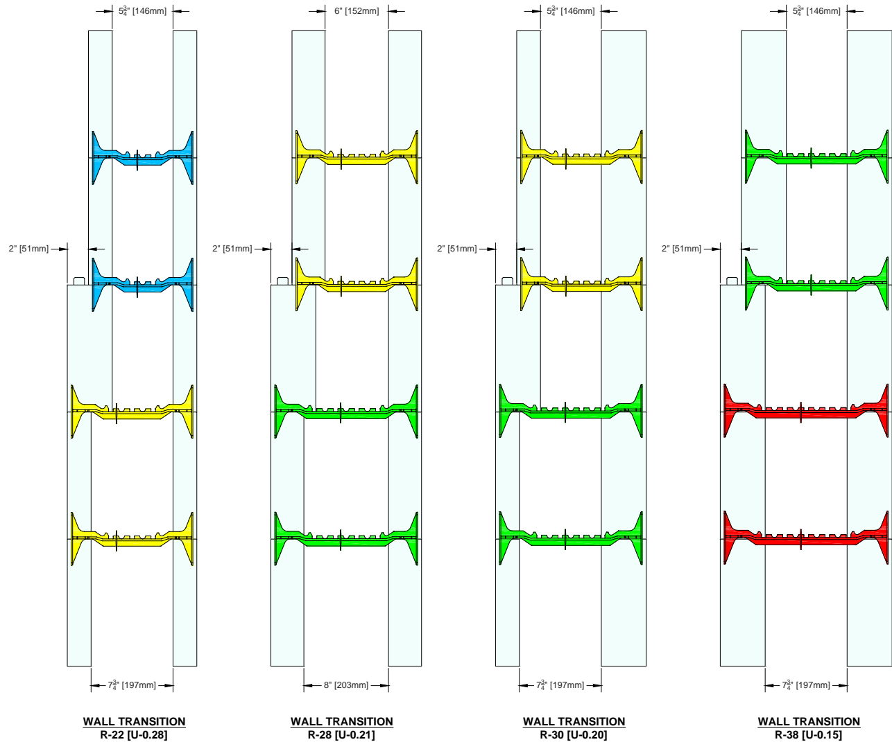
Figure 73: Wall Width Transition using Quad-Lock Plus Panels
