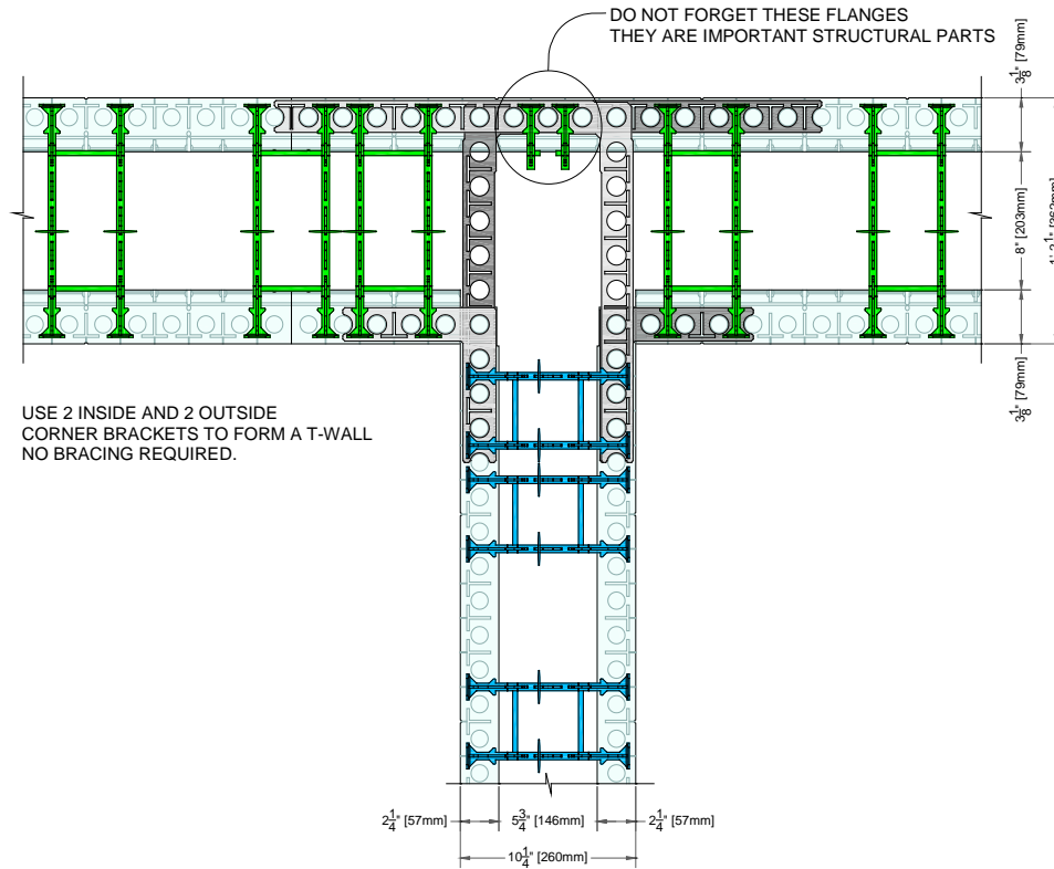
Figure 54: T-Wall Assembly w/ two Outside and two Inside Corner Brackets (plan view)
