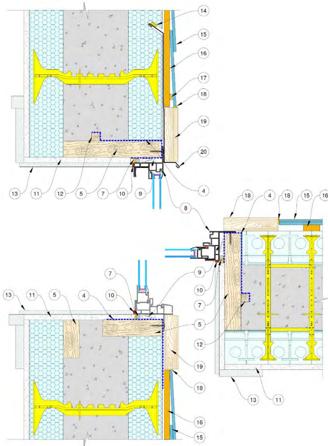
Figure 88: ICF Window Assembly - Wood buck-out, Flanged window flush to exterior, Lapped siding
