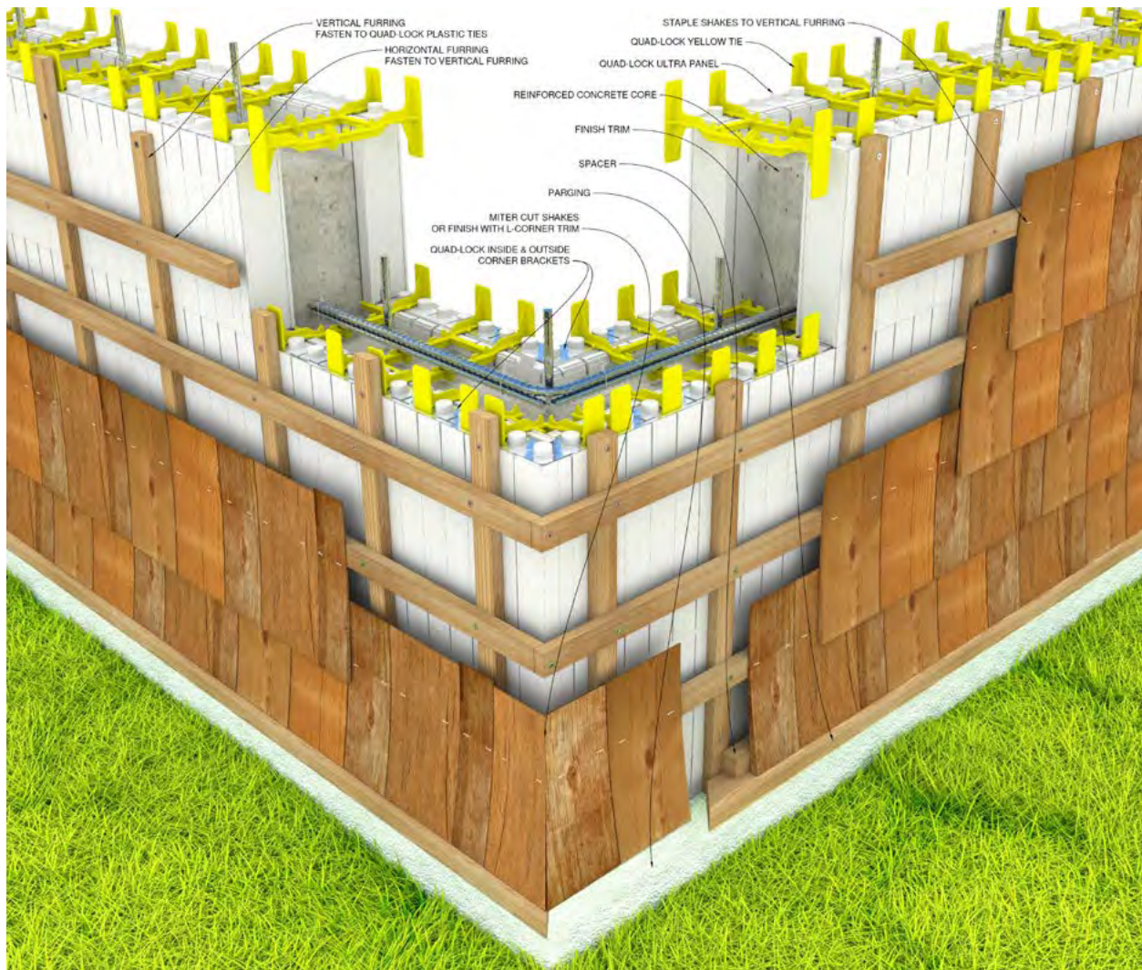
Figure 142: Shake & Shingle finish with external vertical and horizontal furring strips
