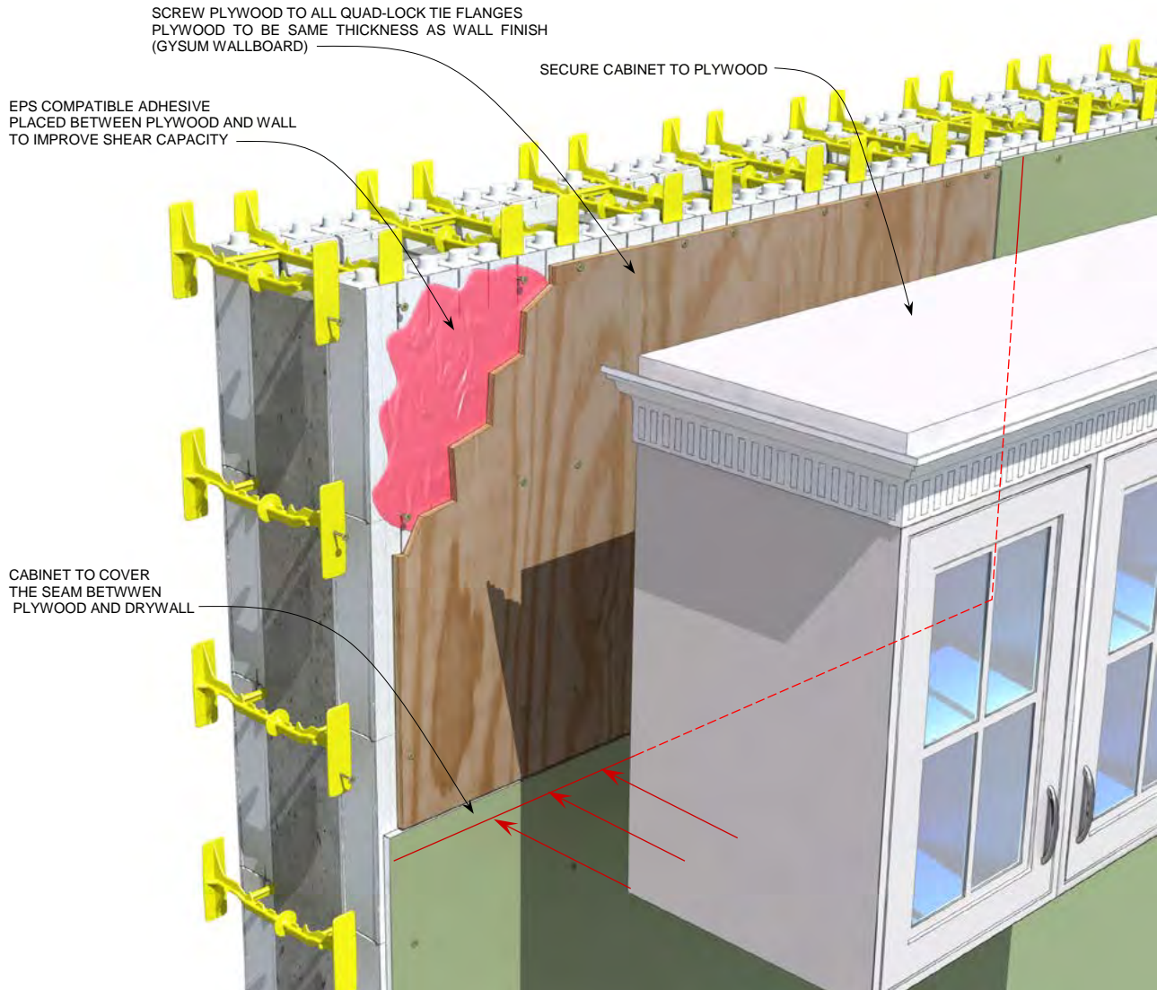
Figure 156: Attaching Heavy Items using Plywood behind Cabinets
