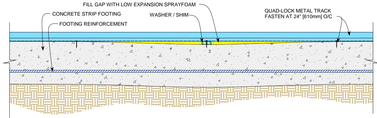
Figure 33: Dealing with Small Variations in Footing Elevations
