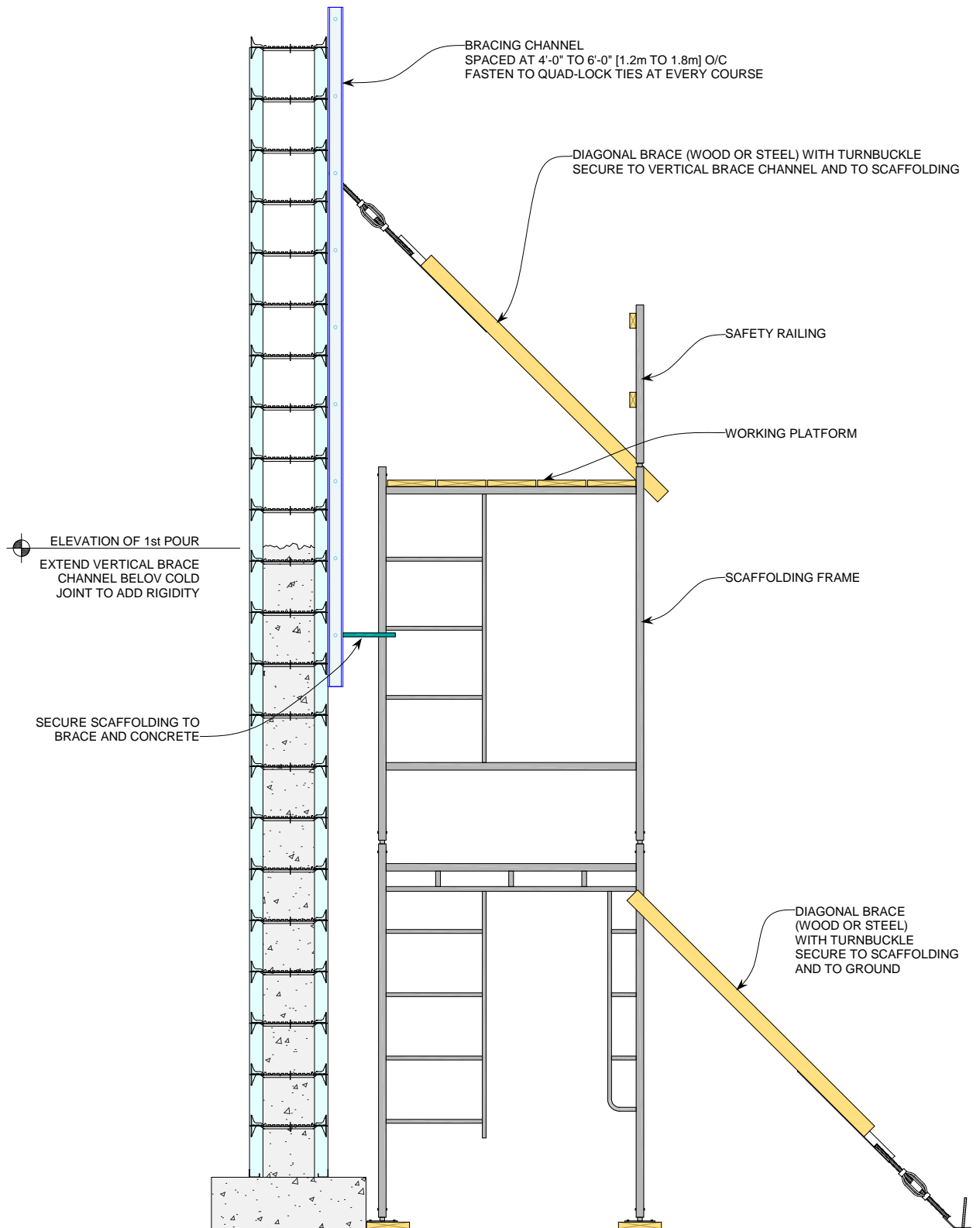
Figure 110: Bracing Tall Walls with Scaffolding
