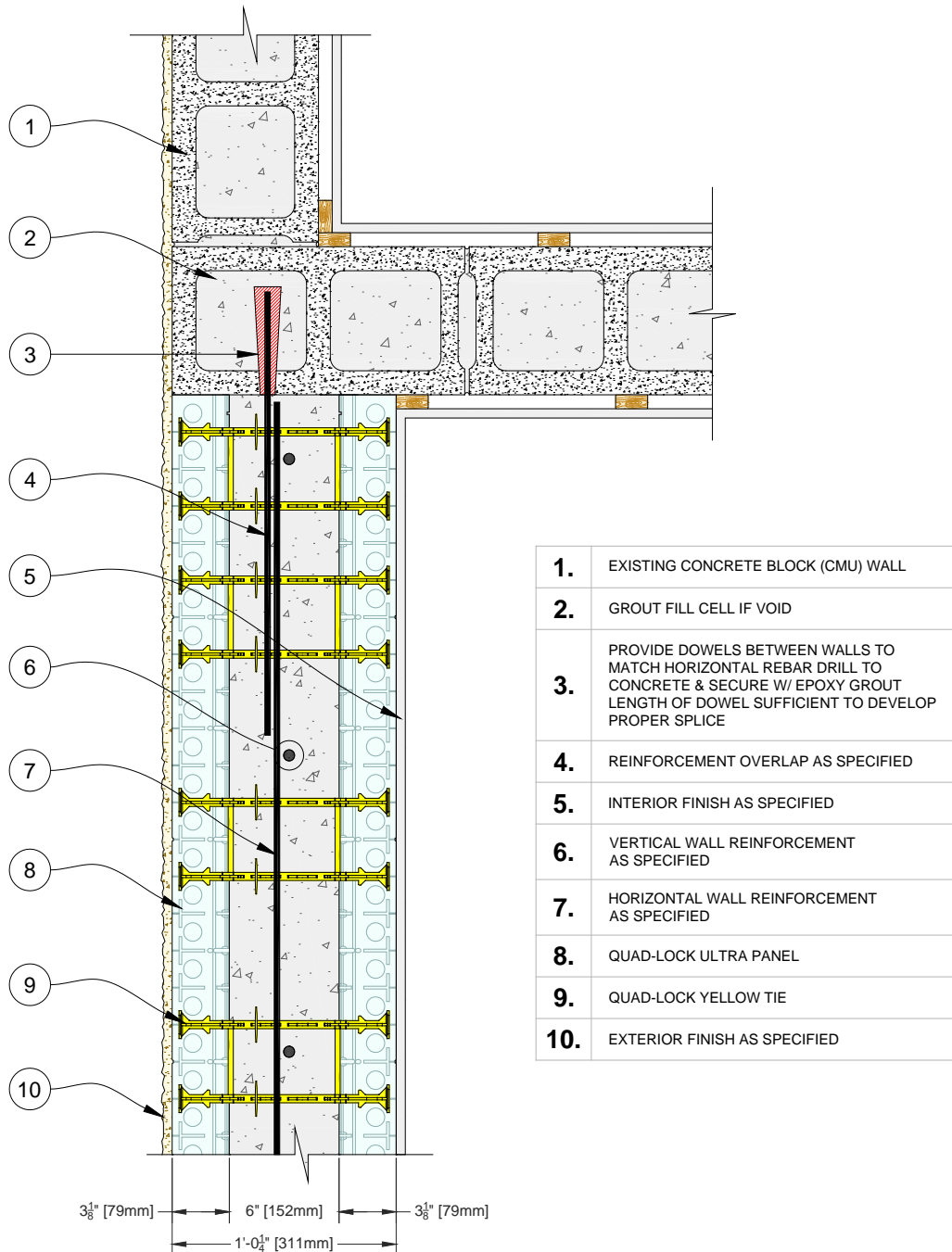
Figure 125: Typical Connection to Existing Concrete Wall (Plan View)
