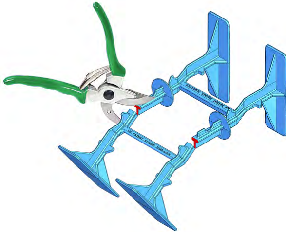
Figure 44: Cut Flanges
