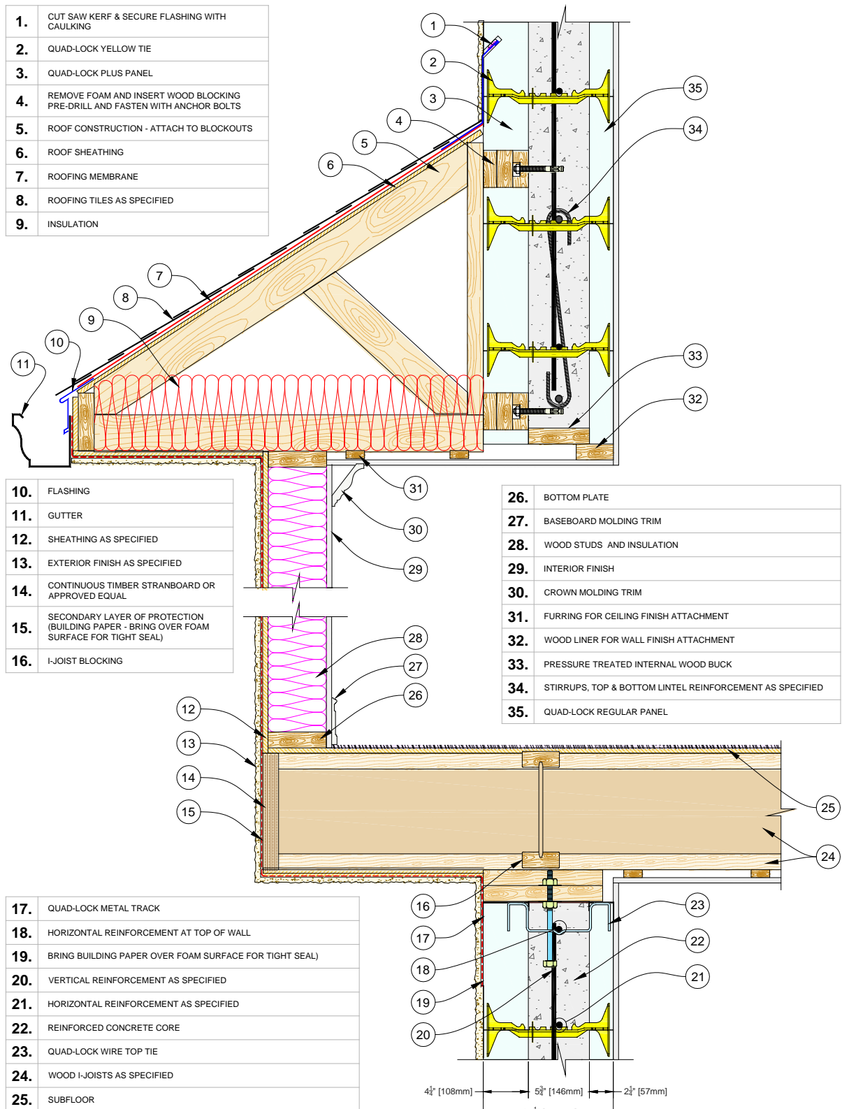
Figure 123: Cantilevered Joist Connection
