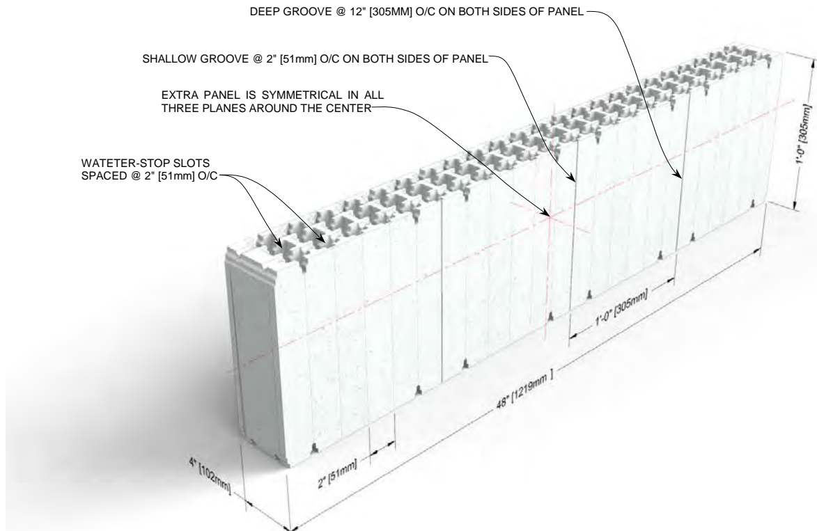
Figure 8: Quad-Lock EXTRA Panel
