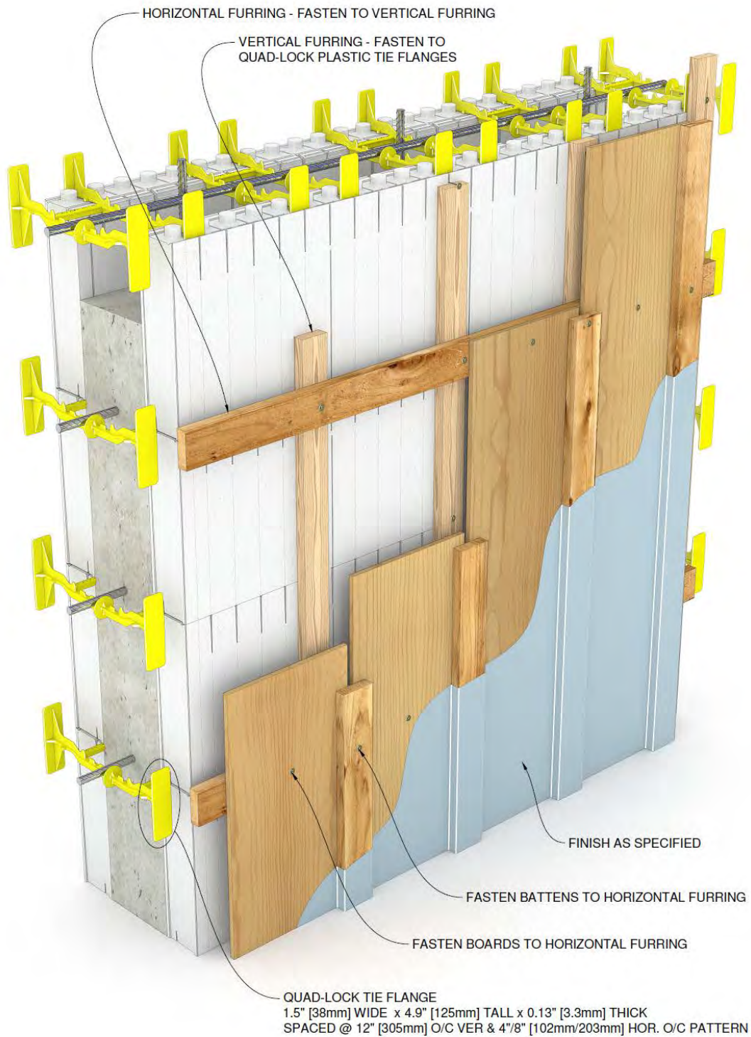
Figure 143: Board & Batten finish with external vertical and horizontal furring strips
