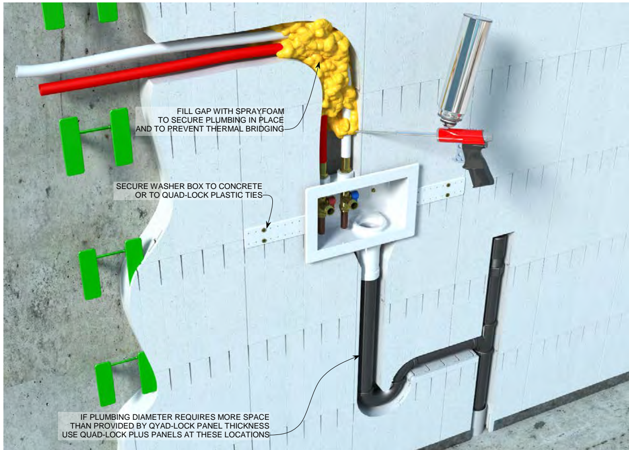
Figure 161: Plumbing Installation (After-Pour Method)
