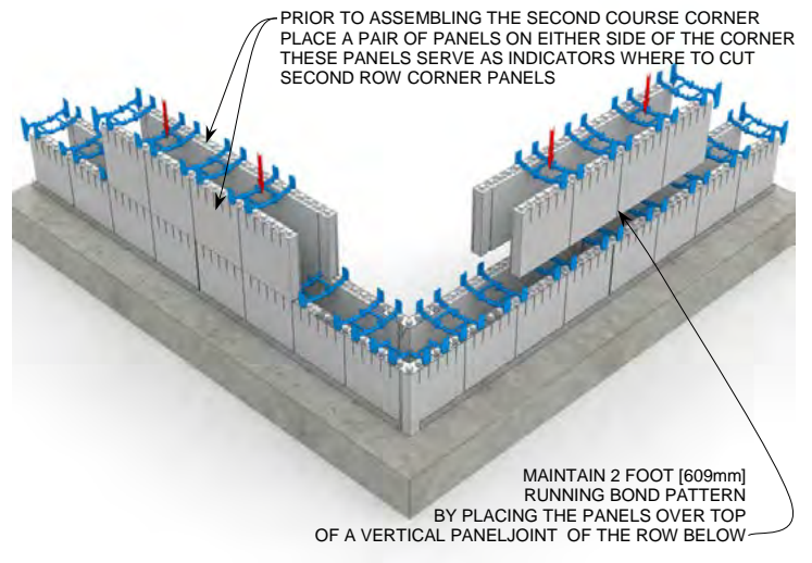
STEP 4 R-22 [U-0.28] 5.75" [146mm] Concrete Wall
