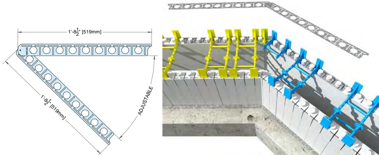
Figure 19: Angle Bracket
