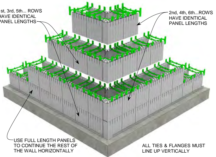
STEP 8 R-30 [U-0.20] 7.75" [197mm] Concrete Wall
