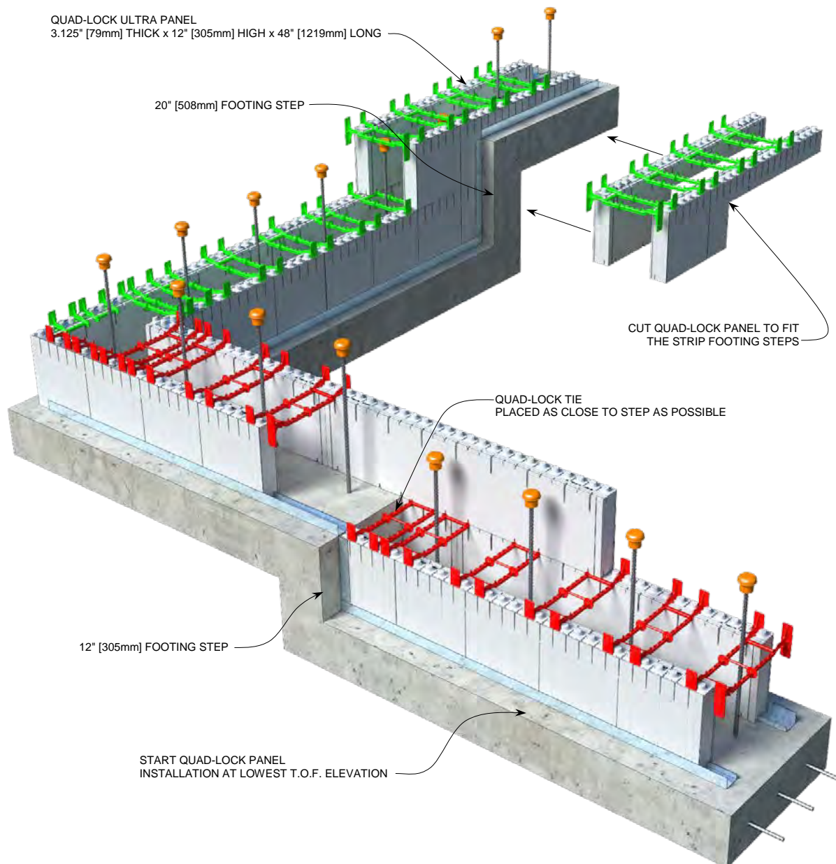
Figure 35: Adapting to Odd Footing Elevations
