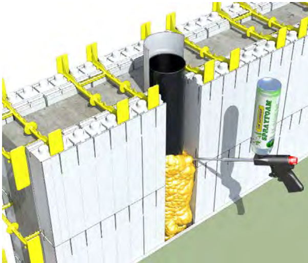
Step 3. Install plumbing, sprayfoam prior to installing wall finish.
