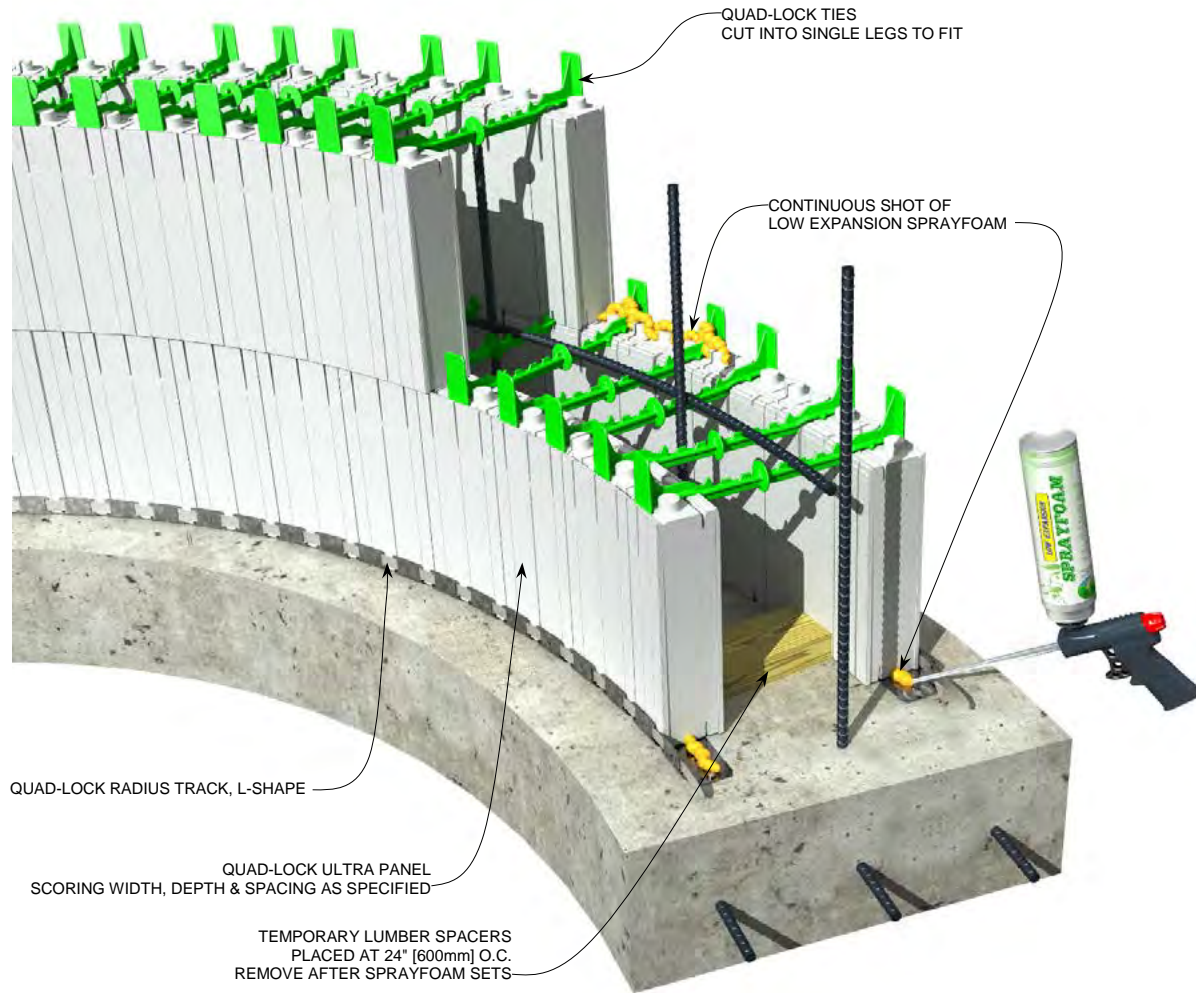
Figure 63: Radius Wall (tight radius)
