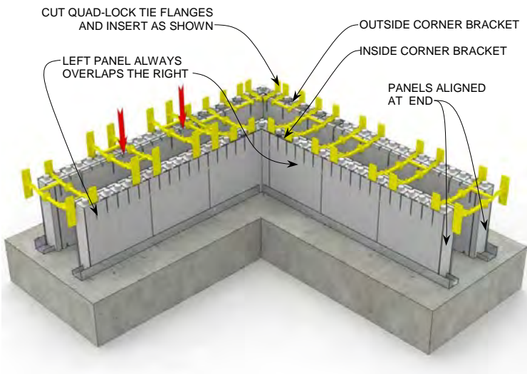
STEP 3 R-28 [U-0.21] 6" [152mm] Concrete Wall (Alternate Method)
