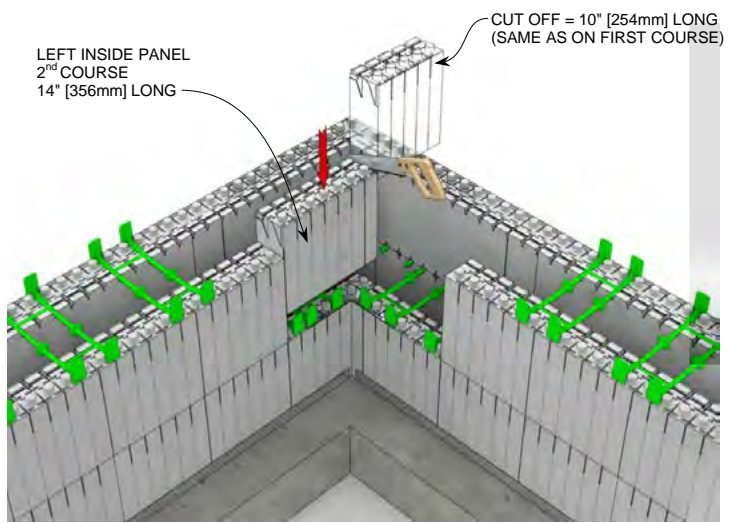
STEP 6 R-38 [U-0.15] 5.75" [146mm] Concrete Wall
