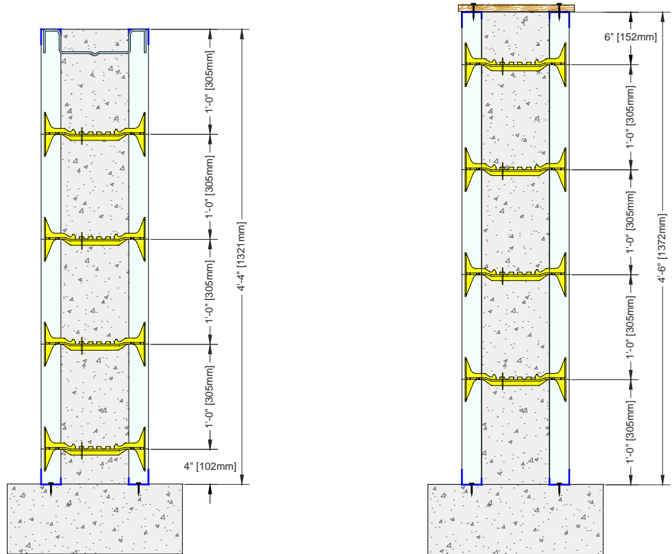
Figure 50: Panels Ripped to Adjust Wall Elevation
