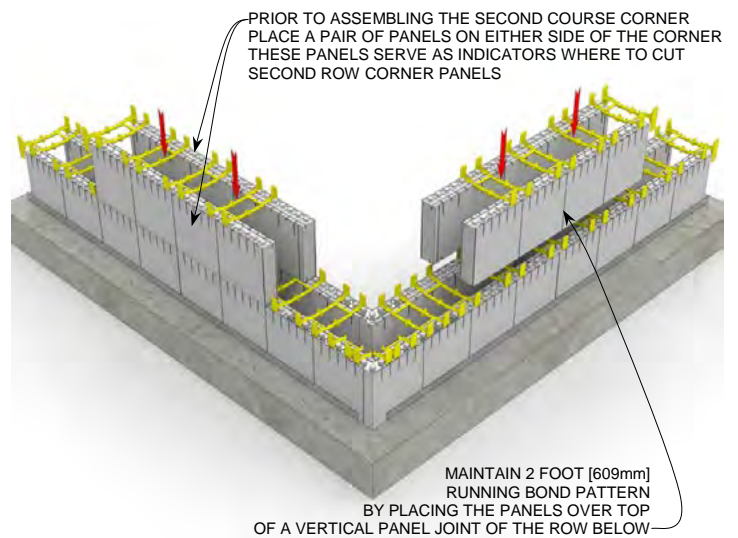
STEP 4 R-28 [U-0.21] 6" [152mm] Concrete Wall
