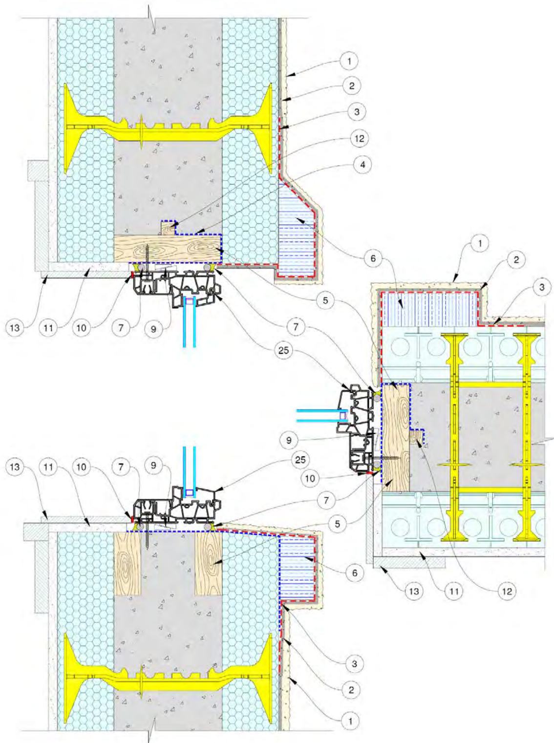
Figure 93: ICF Window Assembly - Wood buck-out, Boxed window centered, EIFS/Stucco lamina
