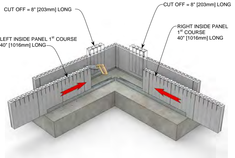
STEP 2 R-22 [U-0.28] 5.75" [146mm] Concrete Wall
