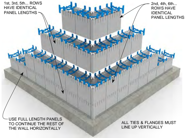
STEP 8 R-22 [U-0.28] 5.75" [146mm] Concrete Wall
