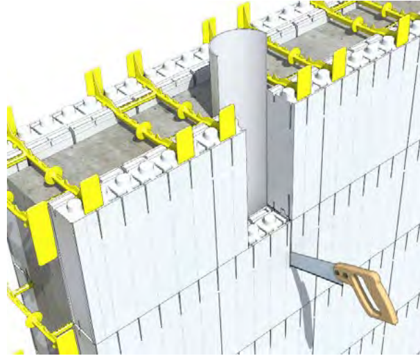
Step 2. Cut out EPS Panels to expose the blocked out area.
