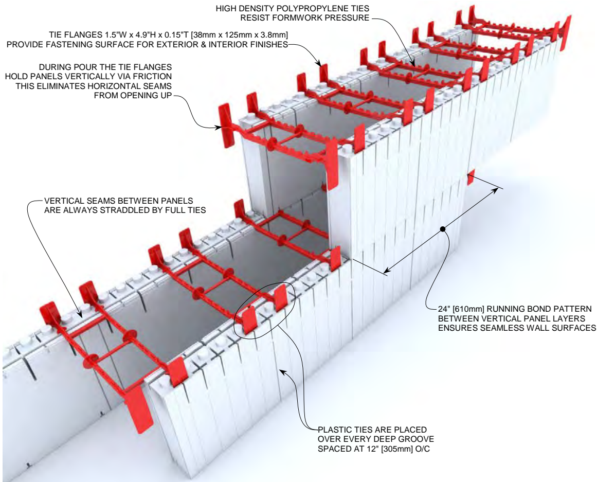
Figure 10: Quad-Lock Ties & Panels
