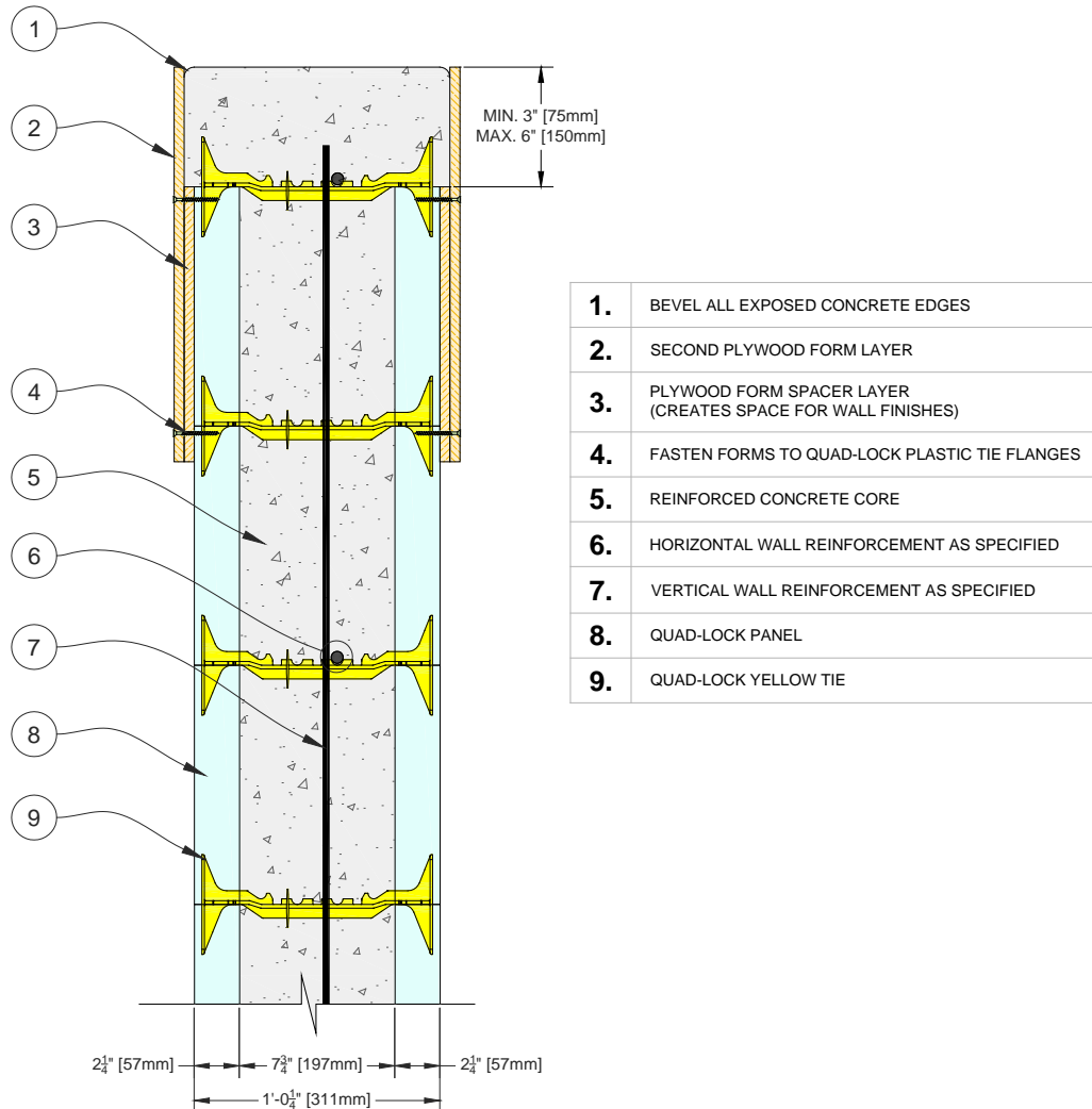
Figure 78: Forming for Solid Wall Cap
