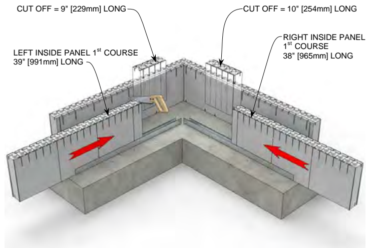
STEP 2 R-28 [U-0.21] 6" [152mm] Concrete Wall (Alternate Method)
