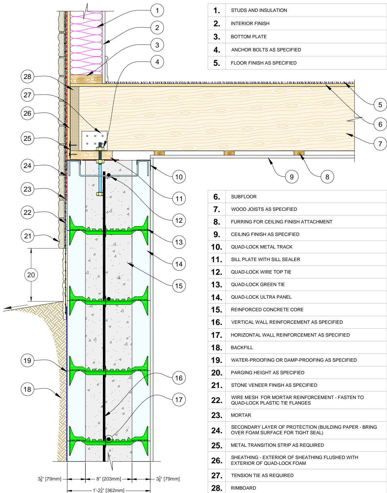
Figure 121: Typical Wall to Floor & Framing Connection
