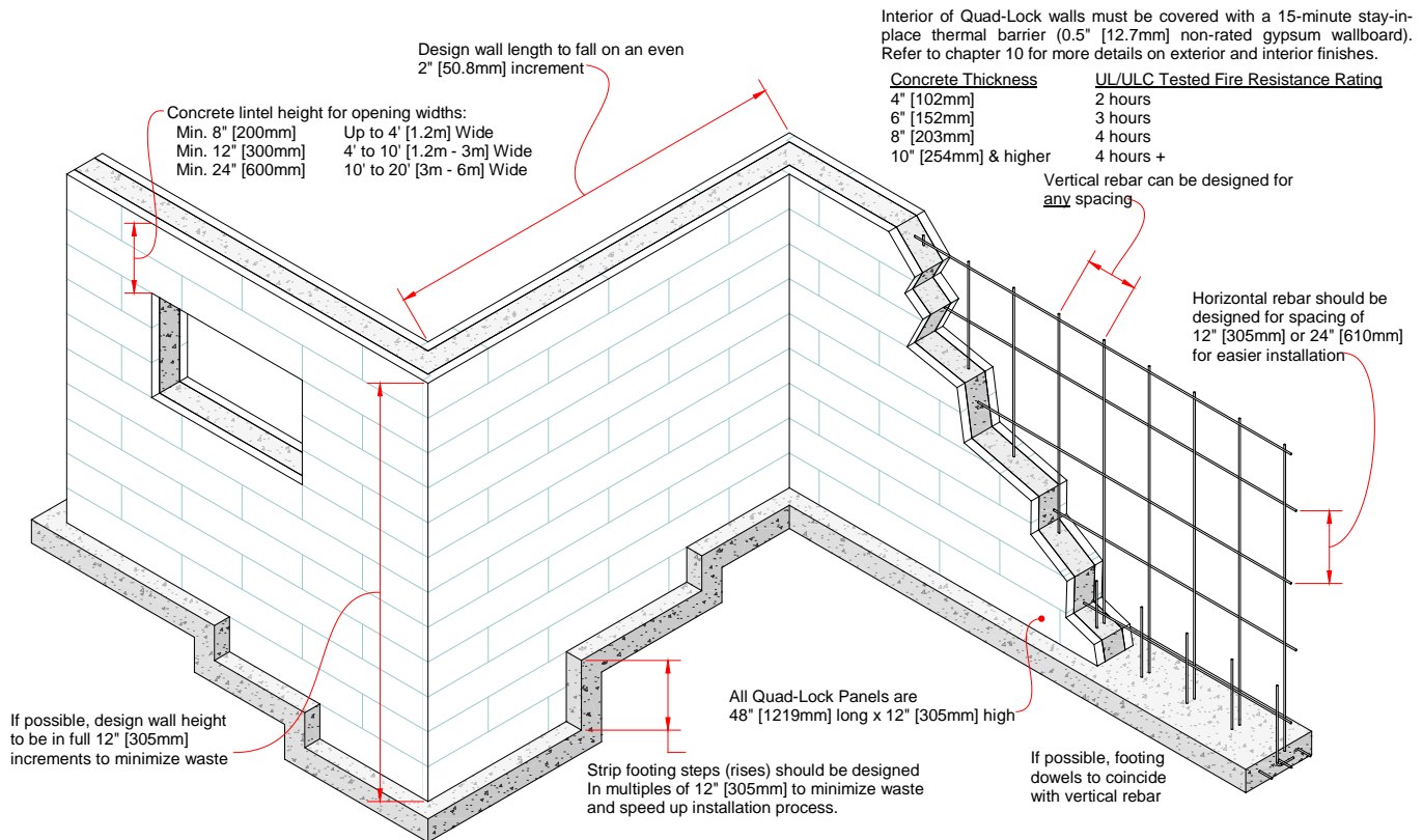
Figure 29: Design Considerations
