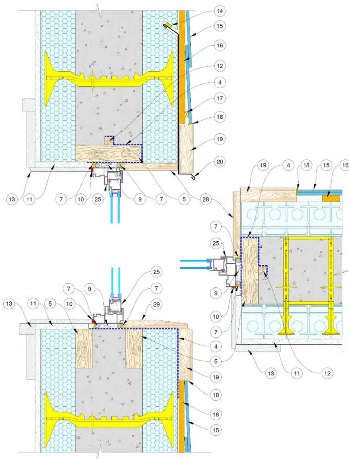
Figure 95: ICF Window Assembly - Wood buck-out, Boxed window centered, Lapped siding
