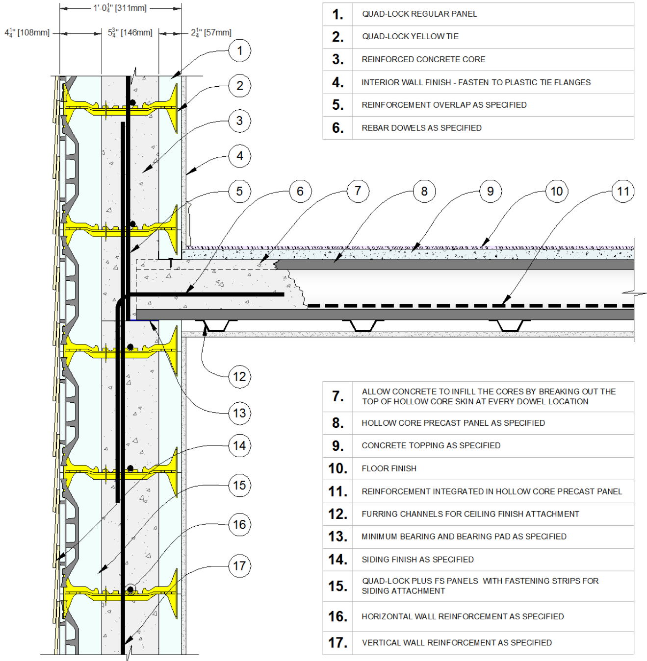
Figure 117: Typical Hollow Core Precast Floor Slab Connection
