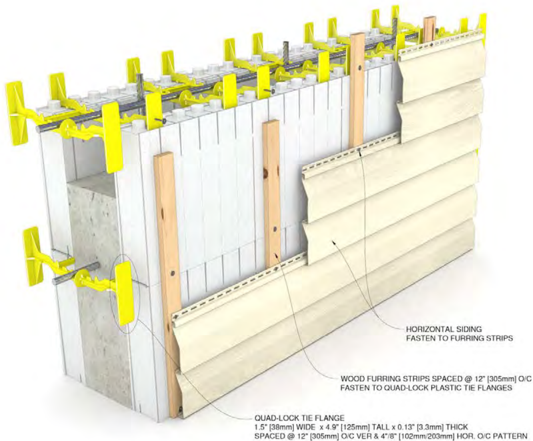
Figure 141: Siding Attachment with external furring strips
