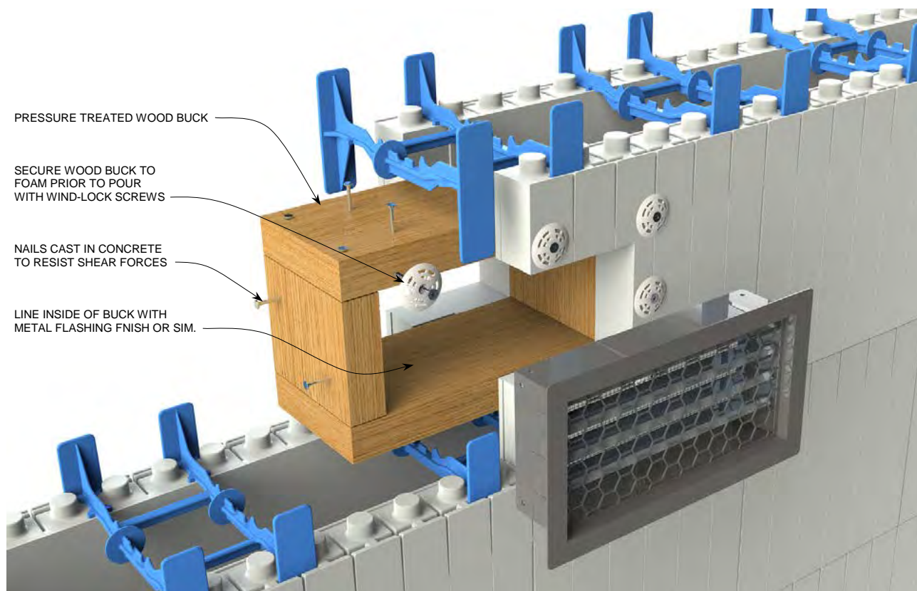
Figure 76: Vent Wall Penetration
