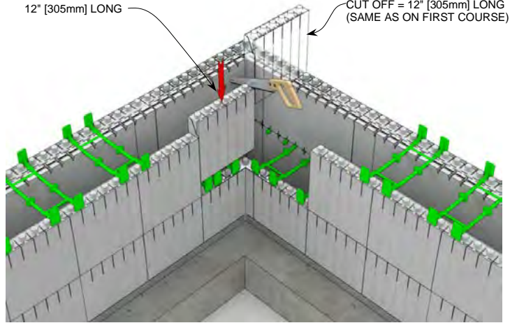
STEP 6 R-30 [U-0.20] 7.75" [197mm] Concrete Wall
