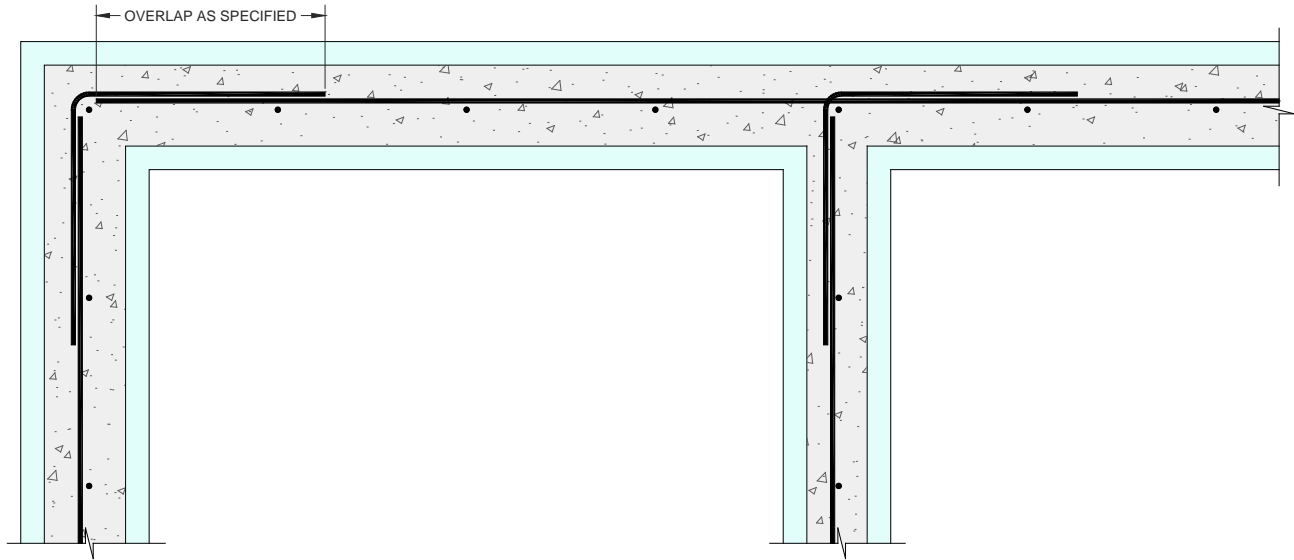
Figure 130: Typical Lap Patterns at Corners & T-Walls
