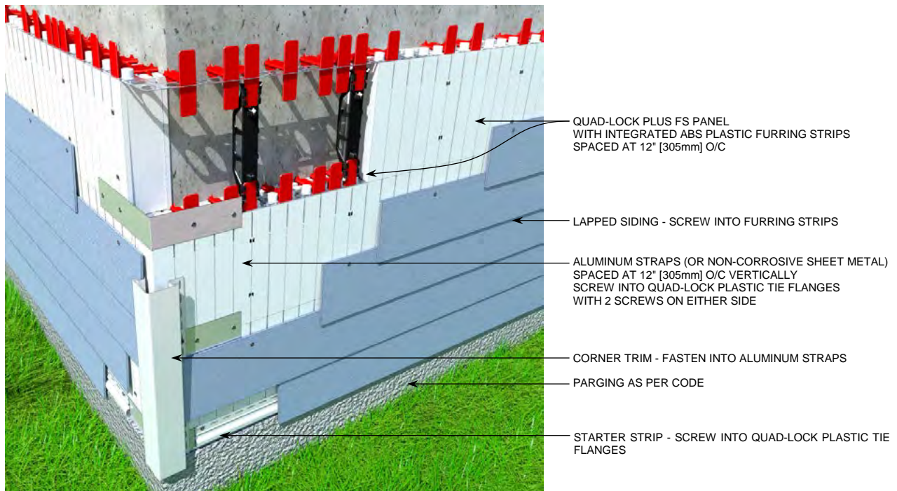
Figure 145: Corner Trim Attachment with Siding Directly Applied to Quad-Lock
