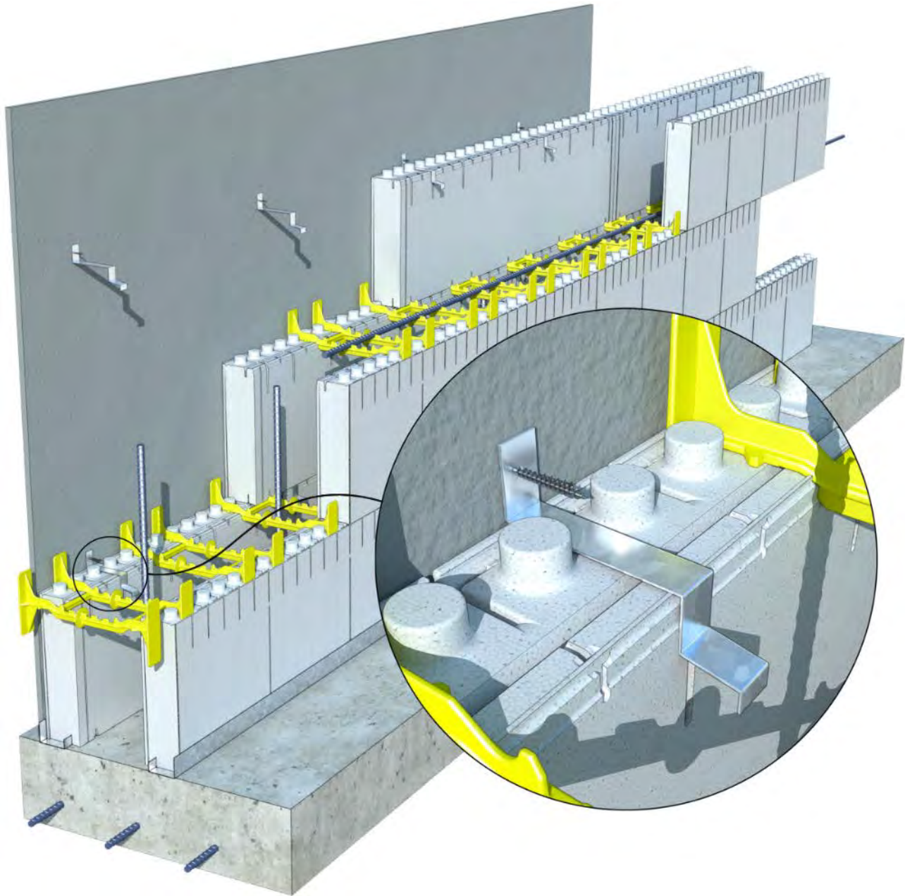
Figure 152: Installing Quad-Lock Walls With no Accesses From Exterior
