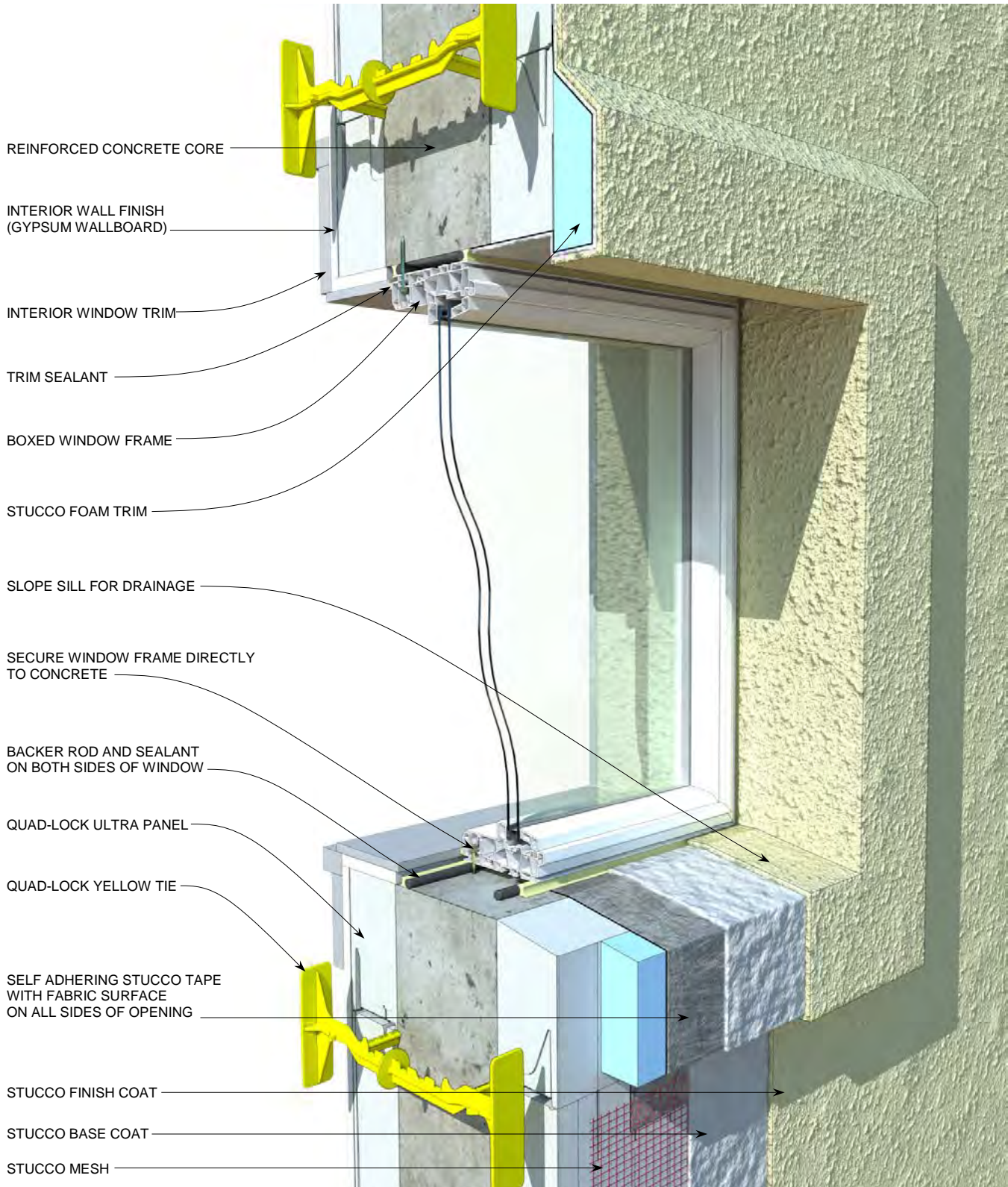
Figure 85: Direct to Concrete Window Assembly
