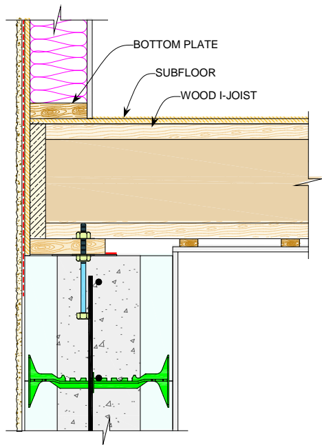
CANTILEVERED PLATE
