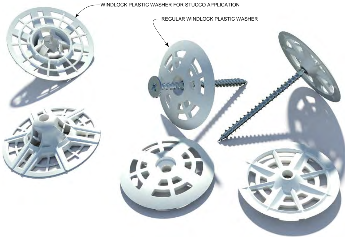
Figure 58: Wind-Lock (Plastic) Washers with Screws
