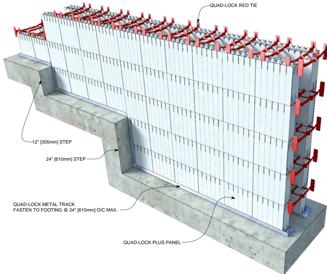
Figure 32: Stepped Footing
