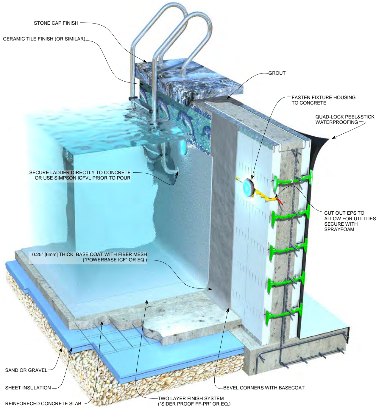
Figure 163: Typical Swimming Pool Wall section
