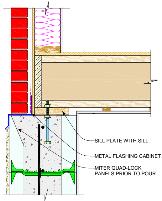
100% BEARING WITH FLASHING
