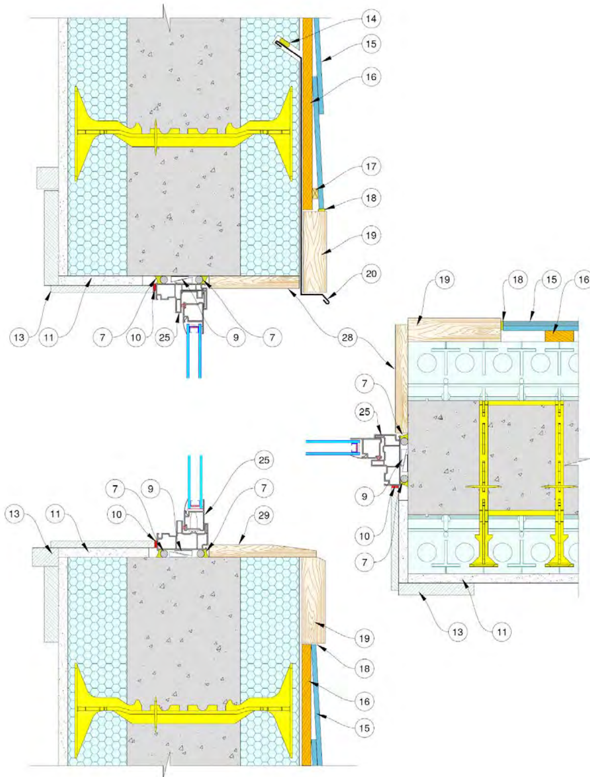
Figure 96: ICF Window Assembly - Direct to concrete, Boxed window centered, Lapped siding
