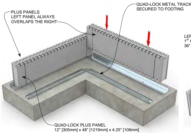
STEP 1 R-30 [U-0.20] 7.75" [197mm] Concrete Wall
