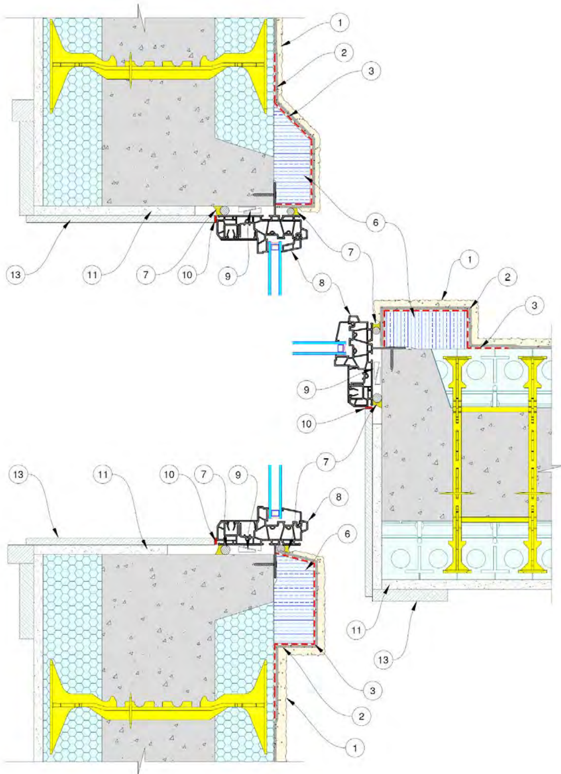
Figure 87: ICF Window Assembly: Direct to concrete, Flanged window flush to exterior, EIFS/Stucco lamina
