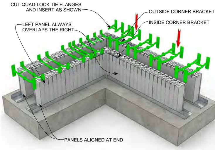
STEP 3 R-38 [U-0.15] 5.75" [146mm] Concrete Wall
