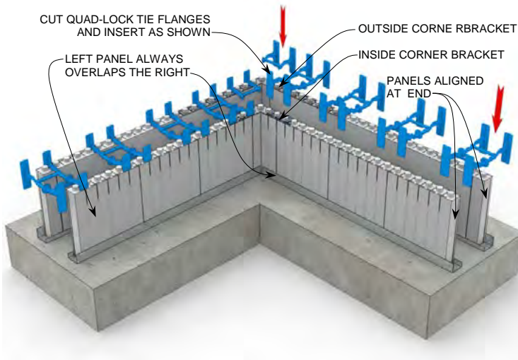
STEP 3 R-22 [U-0.28] 5.75" [146mm] Concrete Wall
