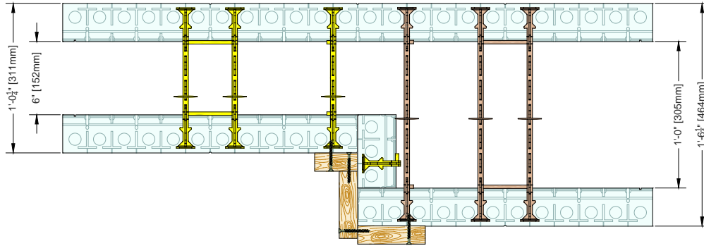
Figure 74: Horizontal (plan view) Wall Width Transition
