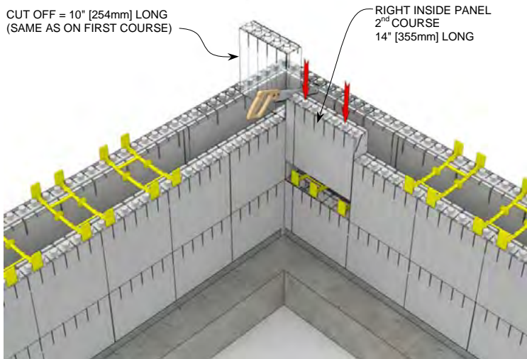
STEP 7 R-28 [U-0.21] 6" [152mm] Concrete Wall
