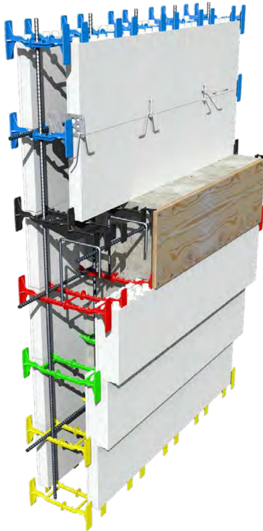
Figure 150: Brick Ledge Formed with Temporary Plywood Forms
