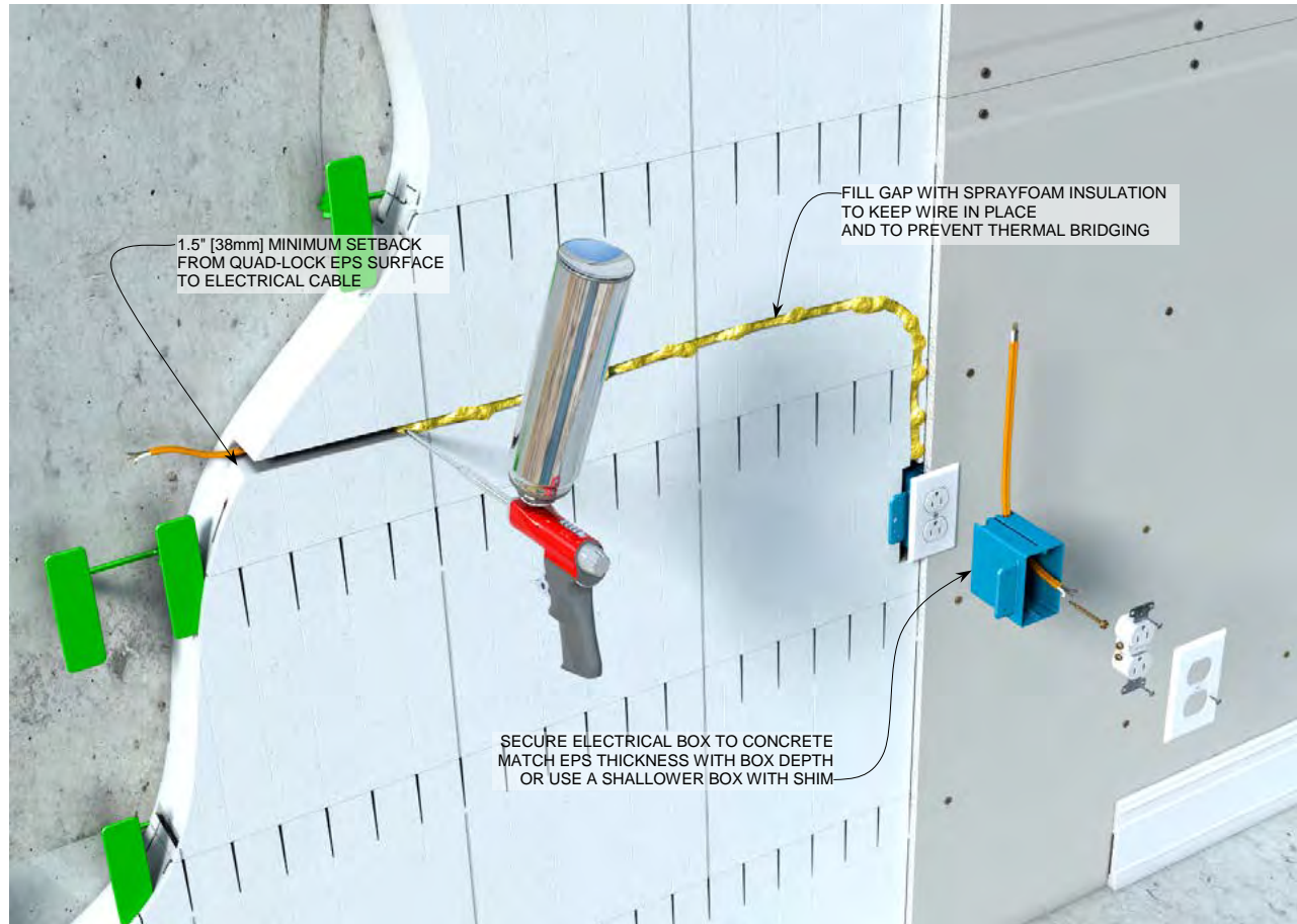
Figure 160: Installation of Electrical Boxes and Wiring
