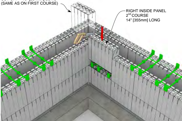
STEP 7 R-38 [U-0.15] 5.75" [146mm] Concrete Wall
