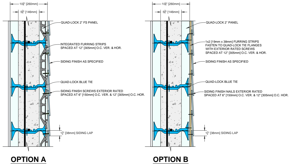
Figure 140: Cladding Detail Options
