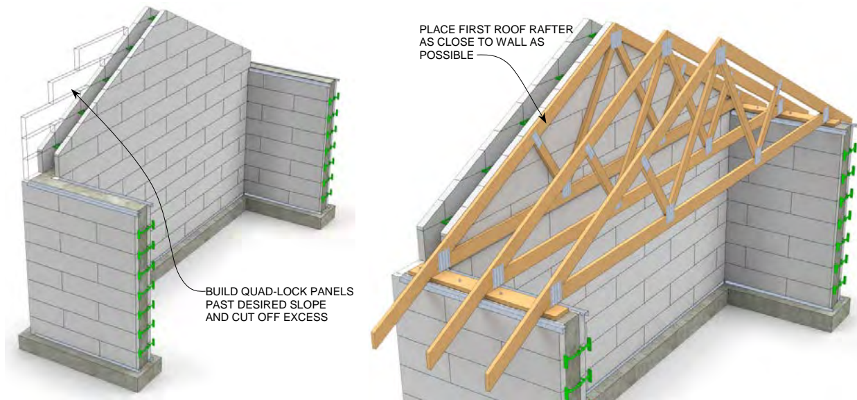
STEP 1 Gable Slope
