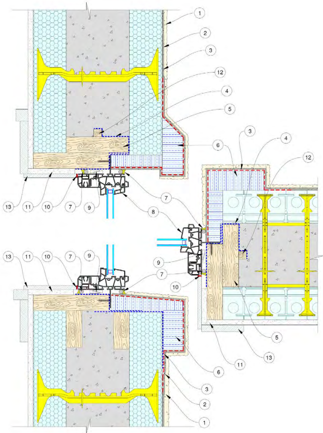
Figure 90: ICF Window Assembly - Wood buck-out, Flanged window centered, EIFS/Stucco lamina
