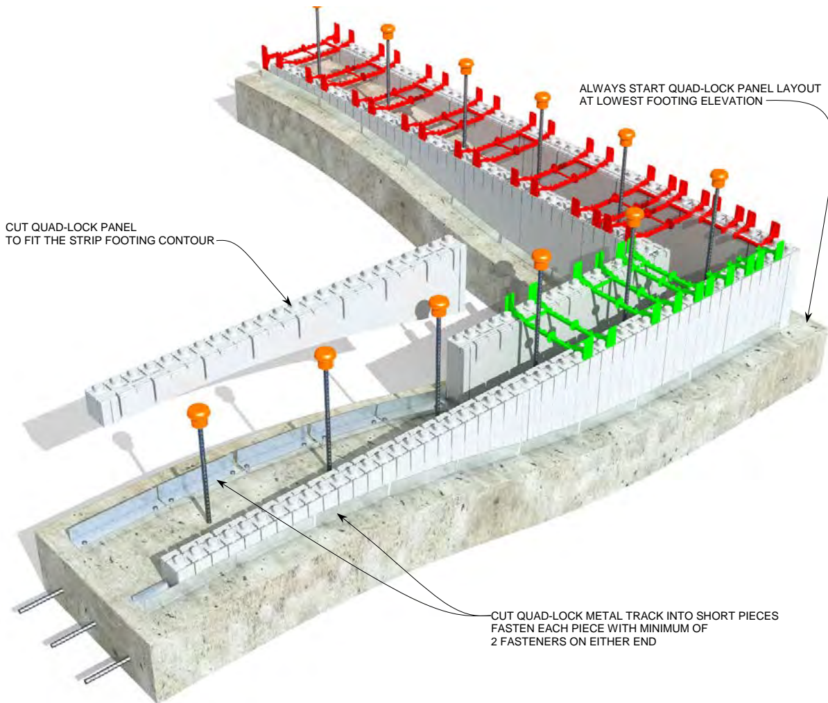
Figure 36: Panels Tapered to Compensate for out-of-level Footing
