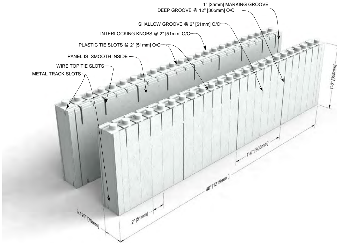
Figure 3: Quad-Lock Ultra Panels
