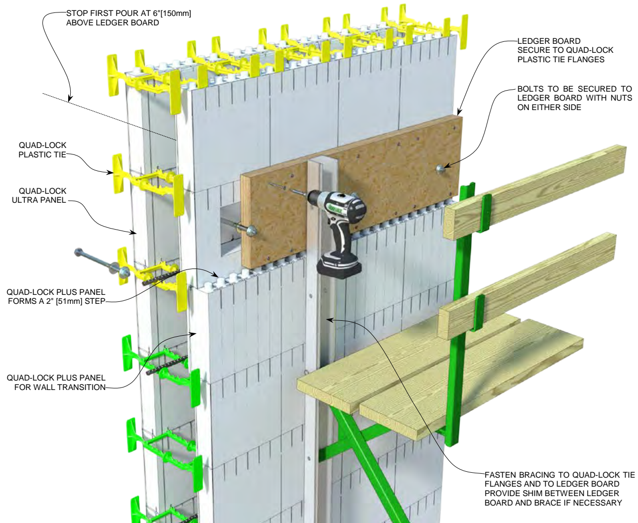
Figure 108: Wall Bracing with Ledger Board in Place
