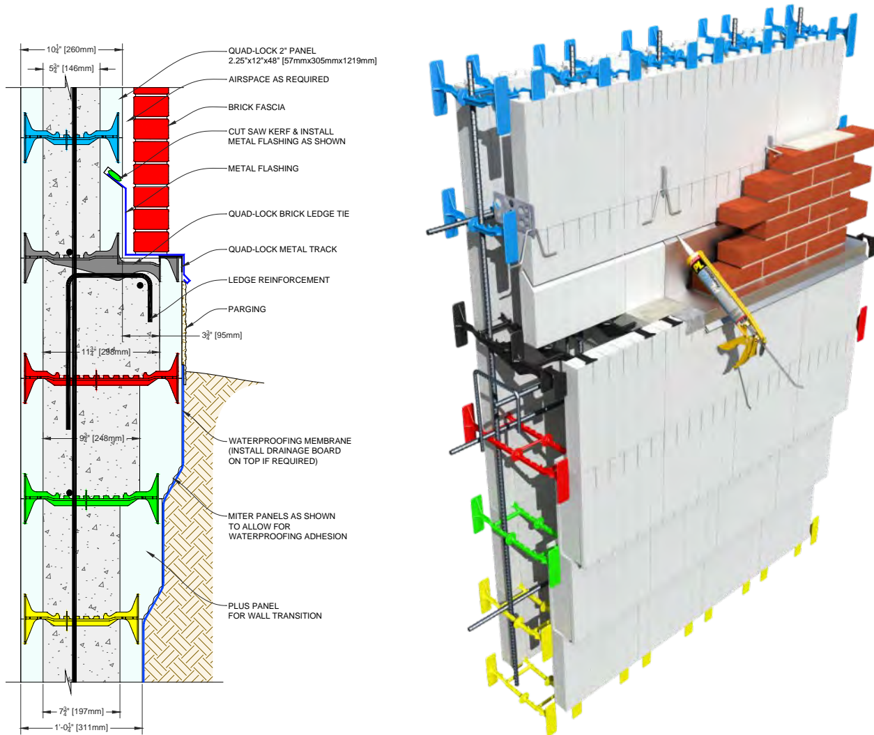
Figure 148: Brick Ledge with Quad-Lock Brick Ledge Tie
