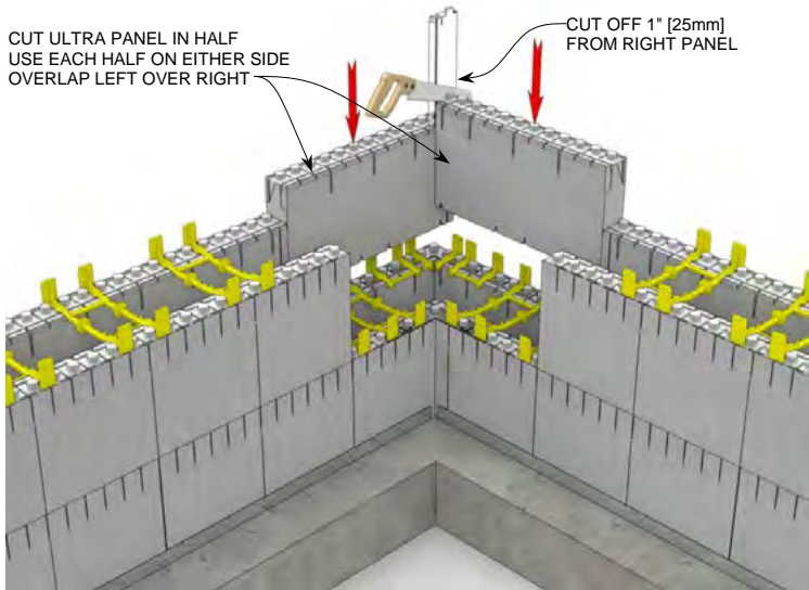
STEP 5 R-28 [U-0.21] 6" [152mm] Concrete Wall (Alternate Method)
