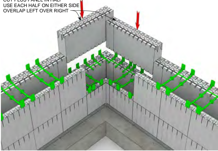
STEP 5 R-30 [U-0.20] 7.75" [197mm] Concrete Wall
