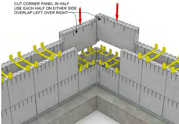
STEP 5 R-28 [U-0.21] 6" [152mm] Concrete Wall
