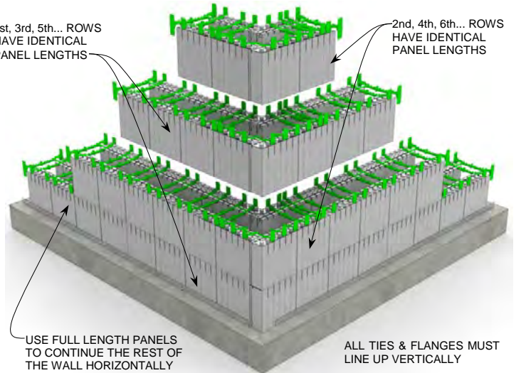
STEP 8 R-38 [U-0.15] 5.75" [146mm] Concrete Wall
