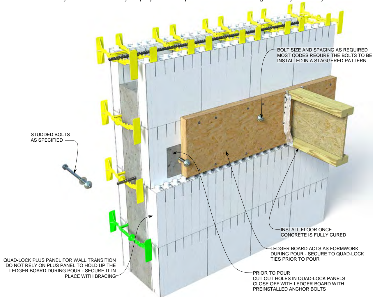
Figure 111: Installation of Floor Ledger Board
