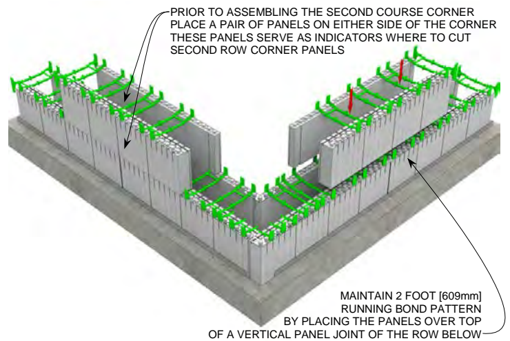
STEP 4 R-30 [U-0.20] 7.75" [197mm] Concrete Wall
