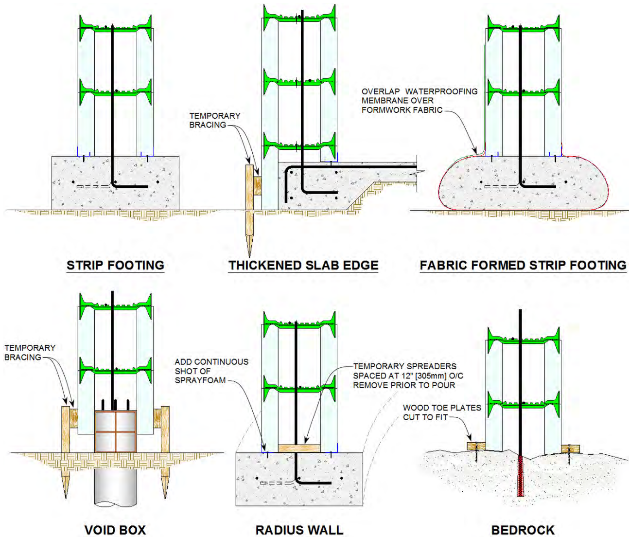
Figure 37: Typical Bottom of Wall Details
