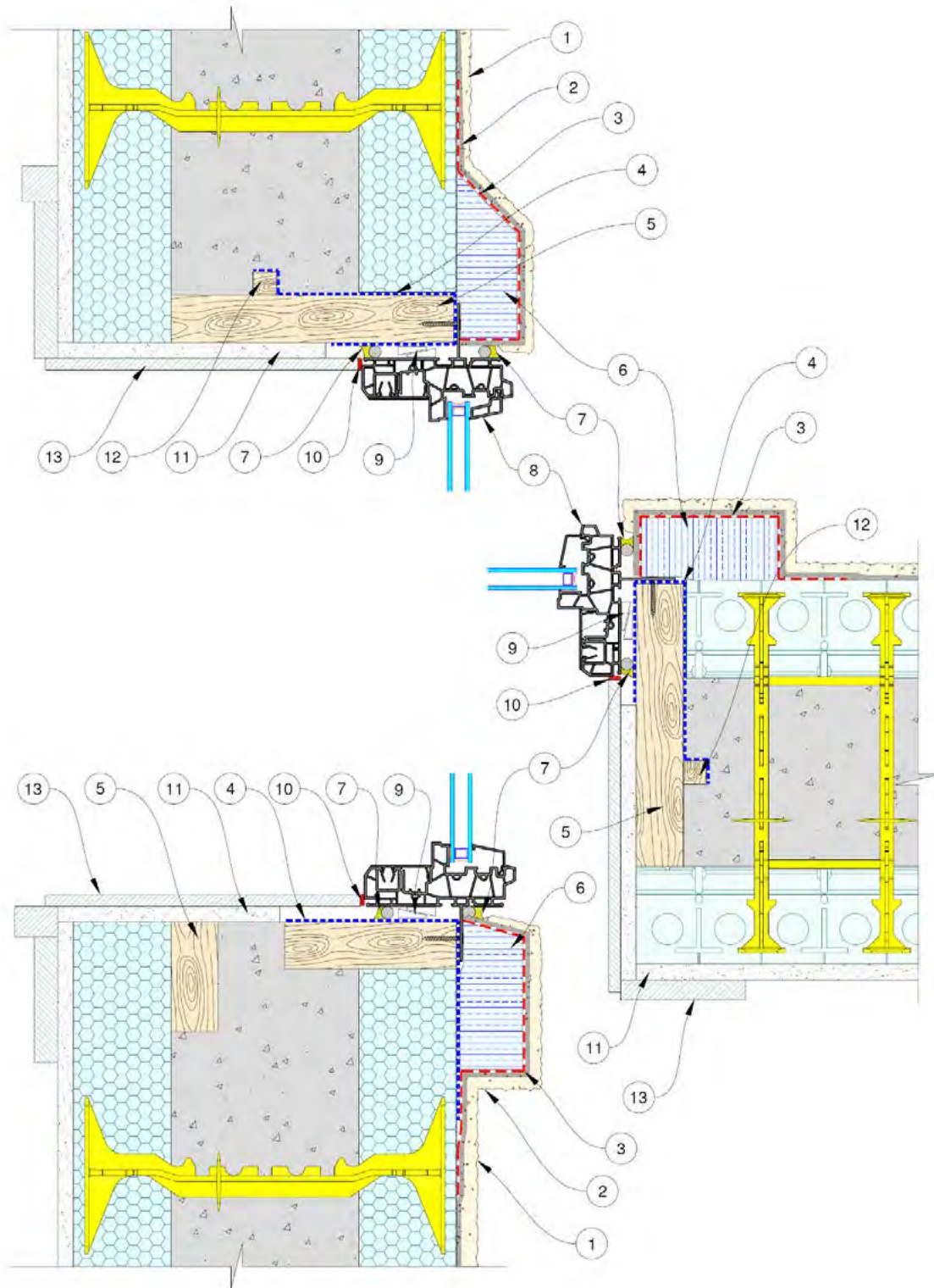
Figure 86: ICF Window Assembly: Wood buck-out, Flanged window flush to exterior, EIFS/Stucco lamina
