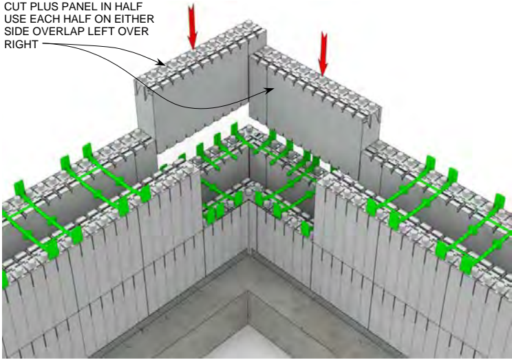
STEP 5 R-38 [U-0.15] 5.75" [146mm] Concrete Wall
