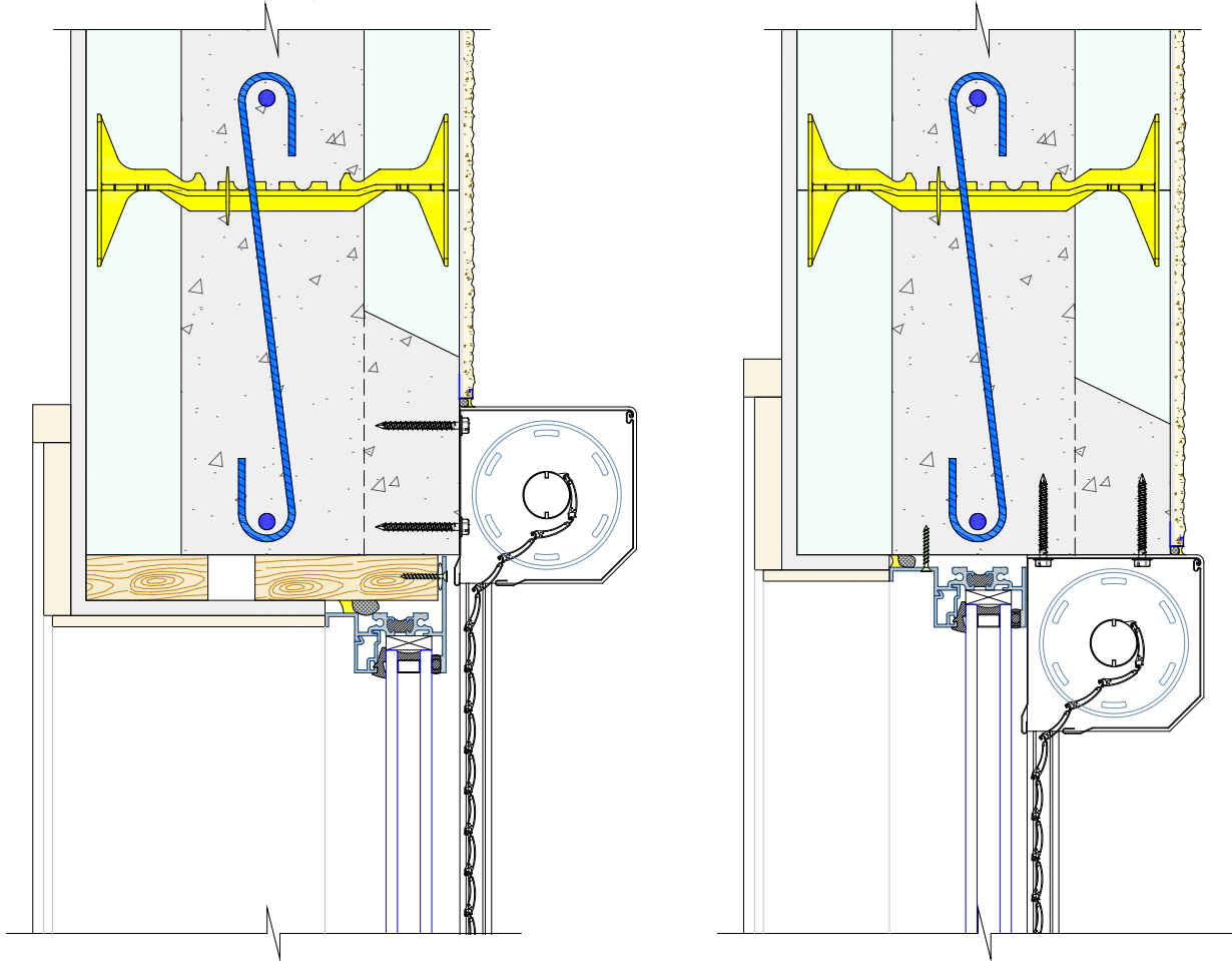
Figure 101: Attachment of Roll-Up Storm Shutter
