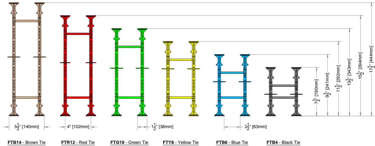
Figure 9: Quad-Lock Standard Ties – Dimensions
