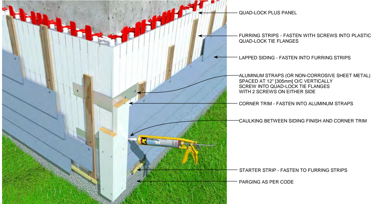
Figure 144: Corner Trim Attachment for Lapped Siding with Rain-Screen
