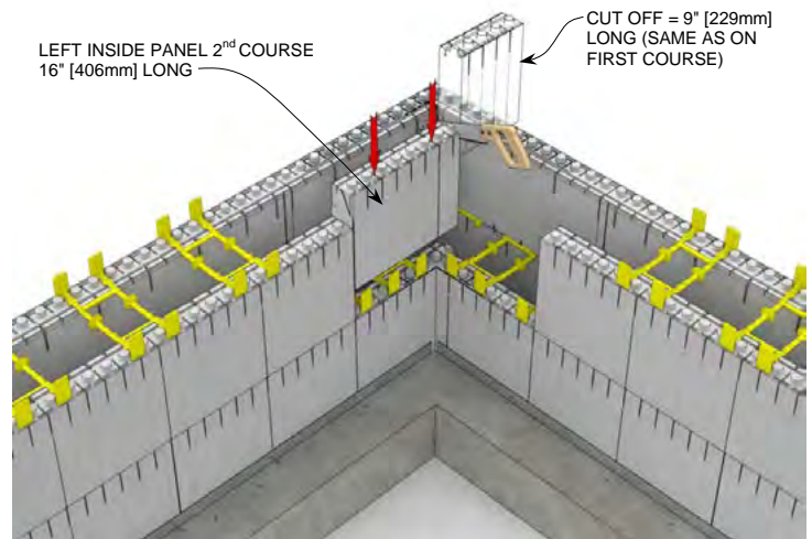
STEP 6 R-28 [U-0.21] 6" [152mm] Concrete Wall
