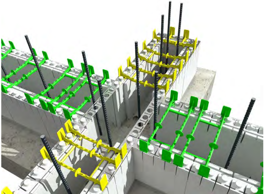
Figure 24: Straight Bracket on T Wall assembly
