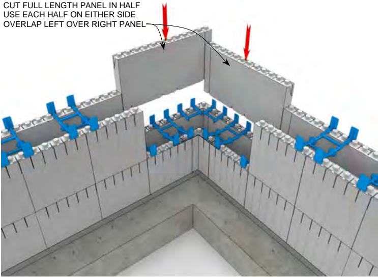
STEP 5 R-22 [U-0.28] 5.75" [146mm] Concrete Wall
