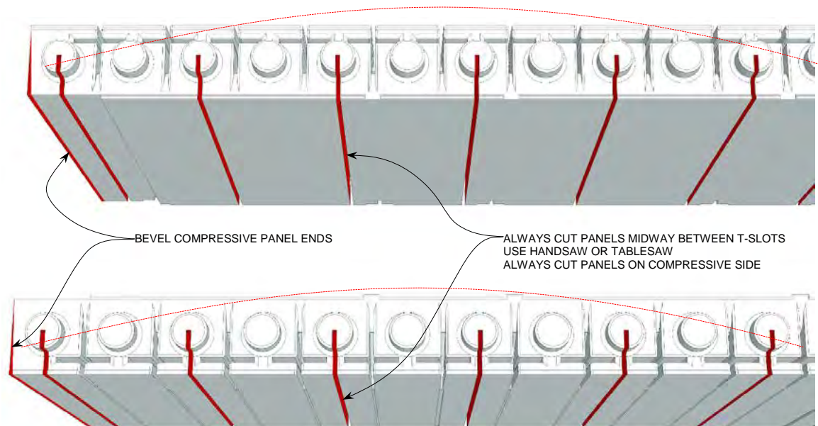
Figure 61: Radius Wall – Panels Cuts
