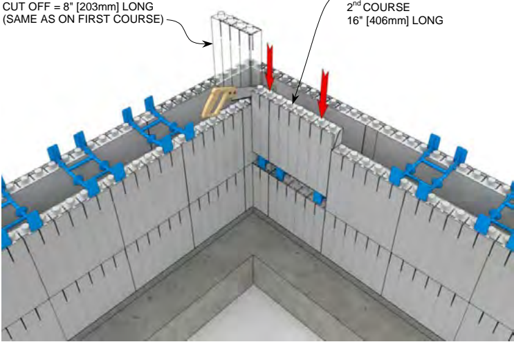
STEP 7 R-22 [U-0.28] 5.75" [146mm] Concrete Wall
