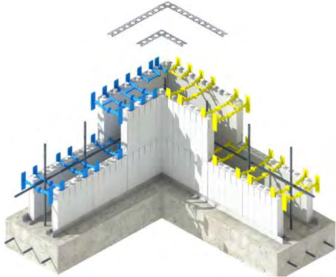
Figure 18: 90° Corner Assembly
