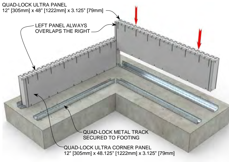
STEP 1 R-28 [U-0.21] 6" [152mm] Concrete Wall
