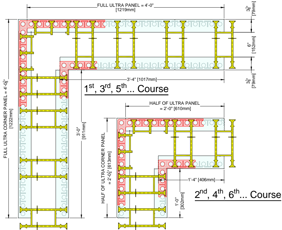
R-28 [U-0.21] CORNER; 6" [152mm] CONCRETE CORE
