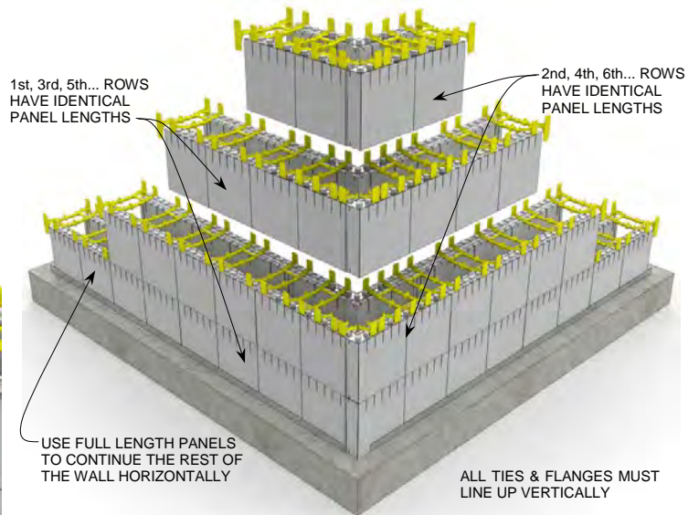
STEP 6 R-28 [U-0.21] 6" [152mm] Concrete Wall (Alternate Method)
