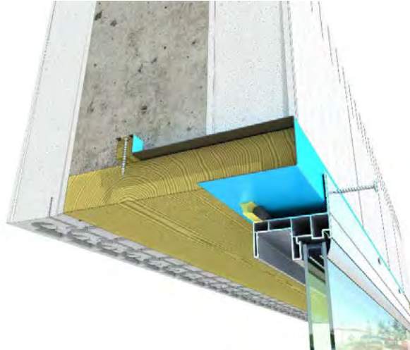
Figure 81: Hybrid Wood Buck-out extends to exterior face of ICF wall
