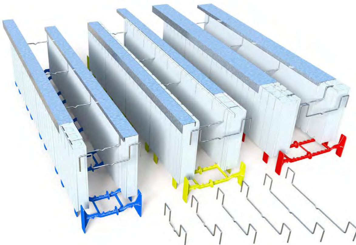
Figure 28: Wire Top Ties used with Metal Track
