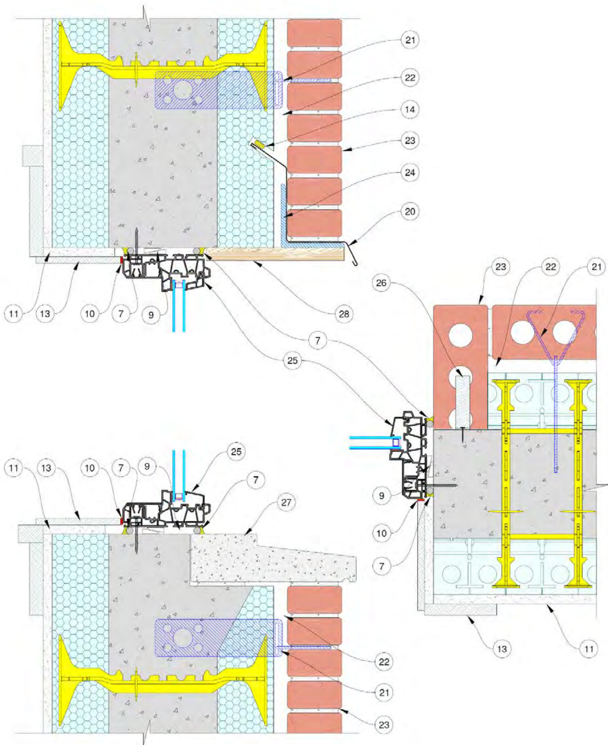
Figure 98: ICF Window Assembly - Direct to concrete, Boxed window centered, Brick veneer
