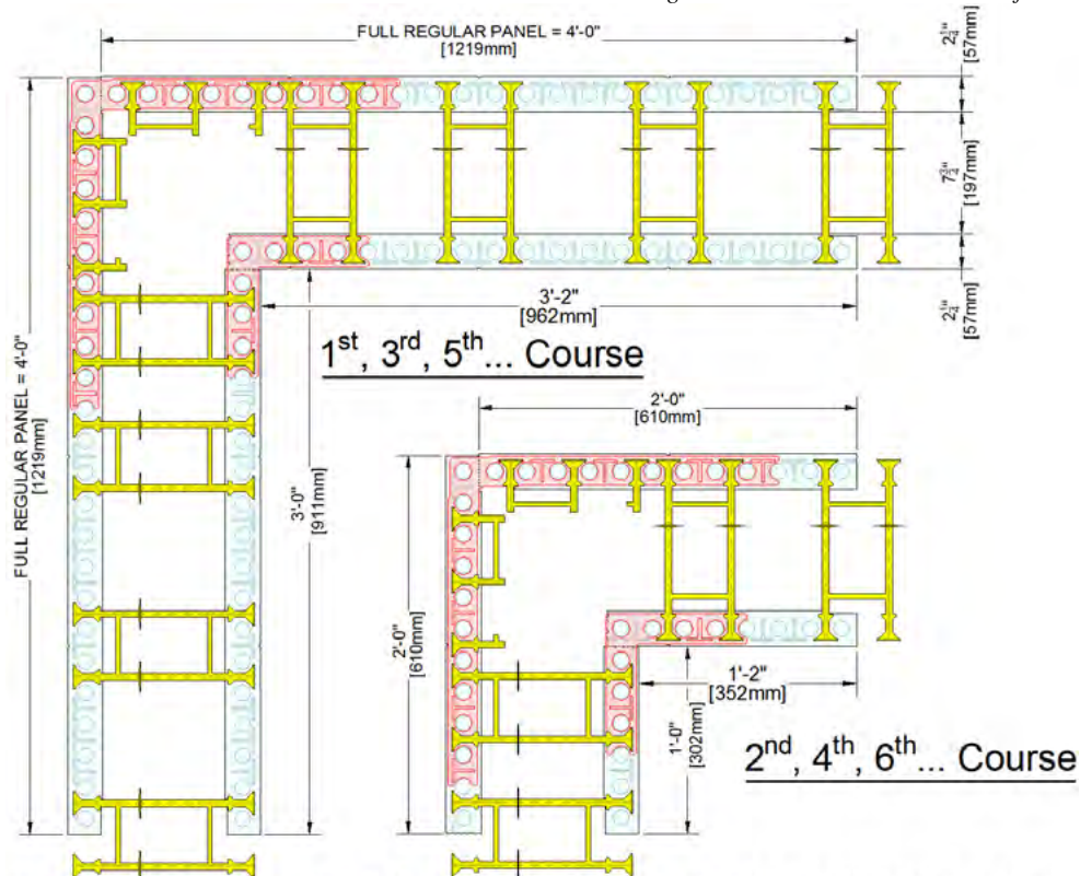
R-22 [U-0.28] CORNER; 7.75" [197mm] CONCRETE CORE
