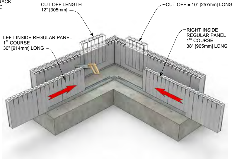
STEP 2 R-30 [U-0.20] 7.75" [197mm] Concrete Wall
