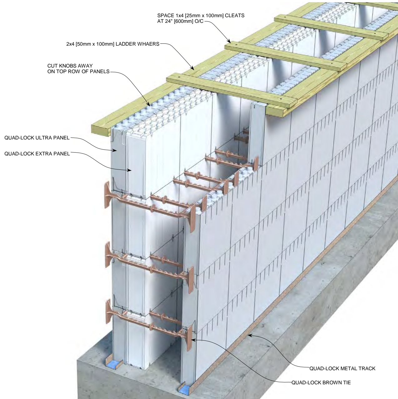
Figure 53: Finishing the Top of Walls with wood Ladder brace
