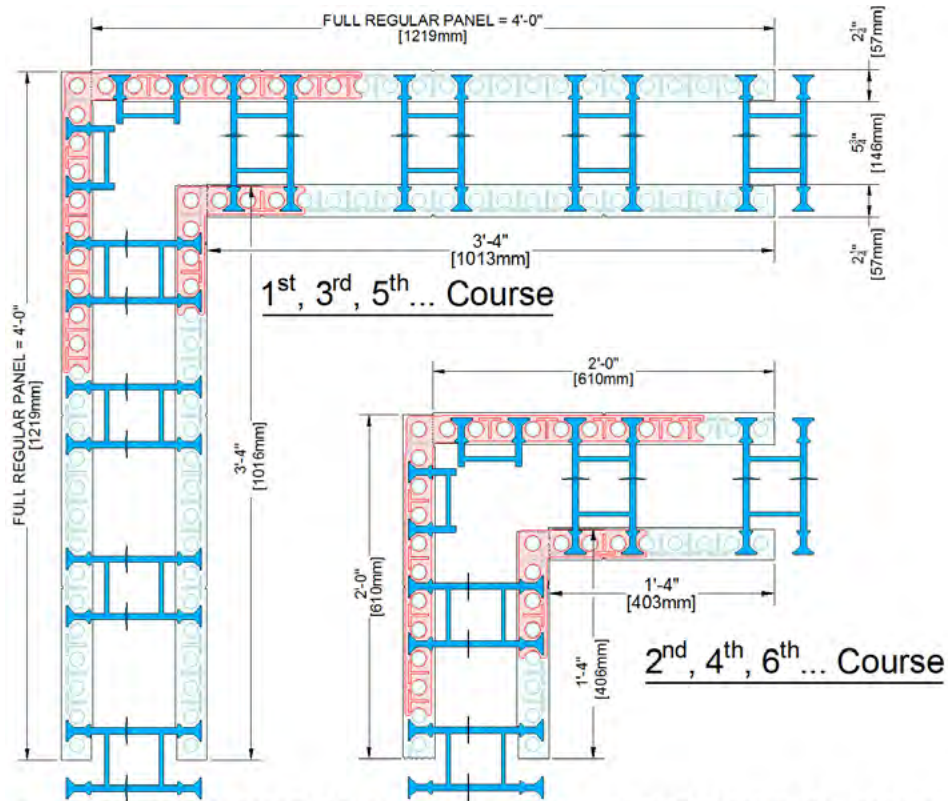
R-22 [U-0.28] CORNER; 5.75" [146mm] CONCRETE CORE
