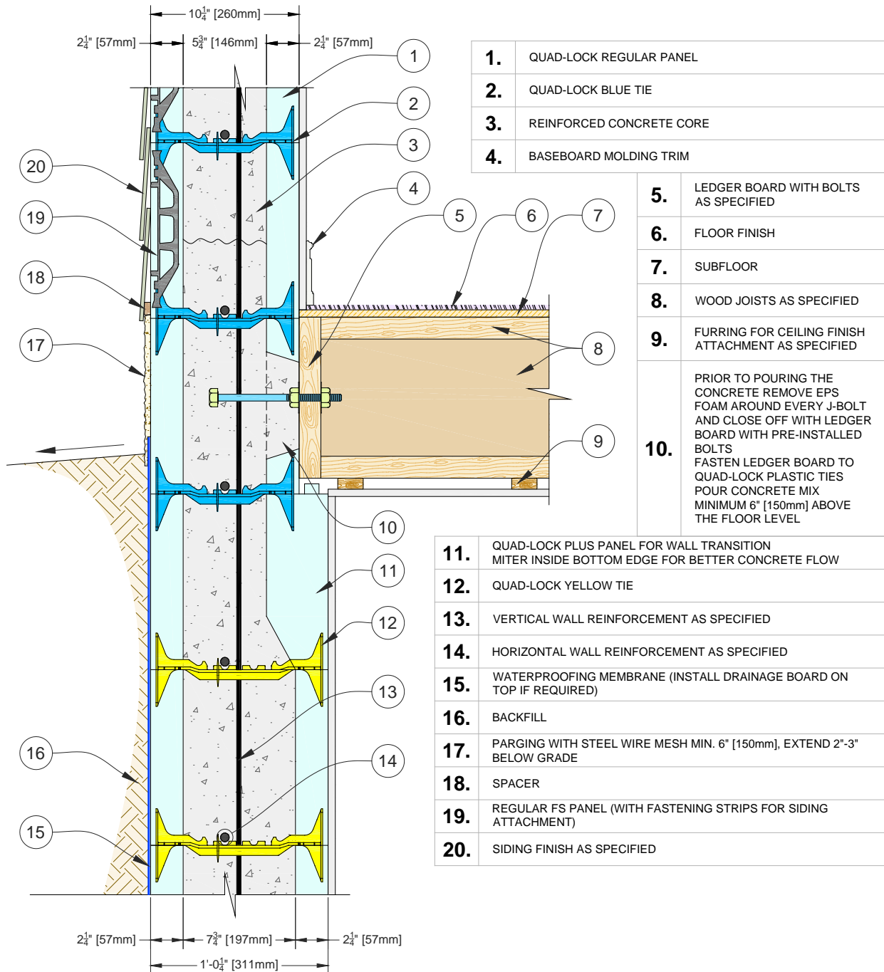
Figure 72: Wall Width Transition & Ledger Connection
