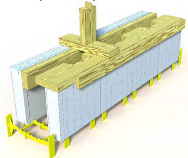
Hybrid Sill - Cut out holes to provide access for pouring
