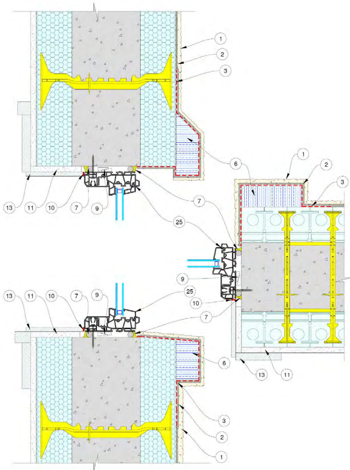
Figure 94: ICF Window Assembly - Direct to concrete, Boxed window centered, EIFS/Stucco lamina
