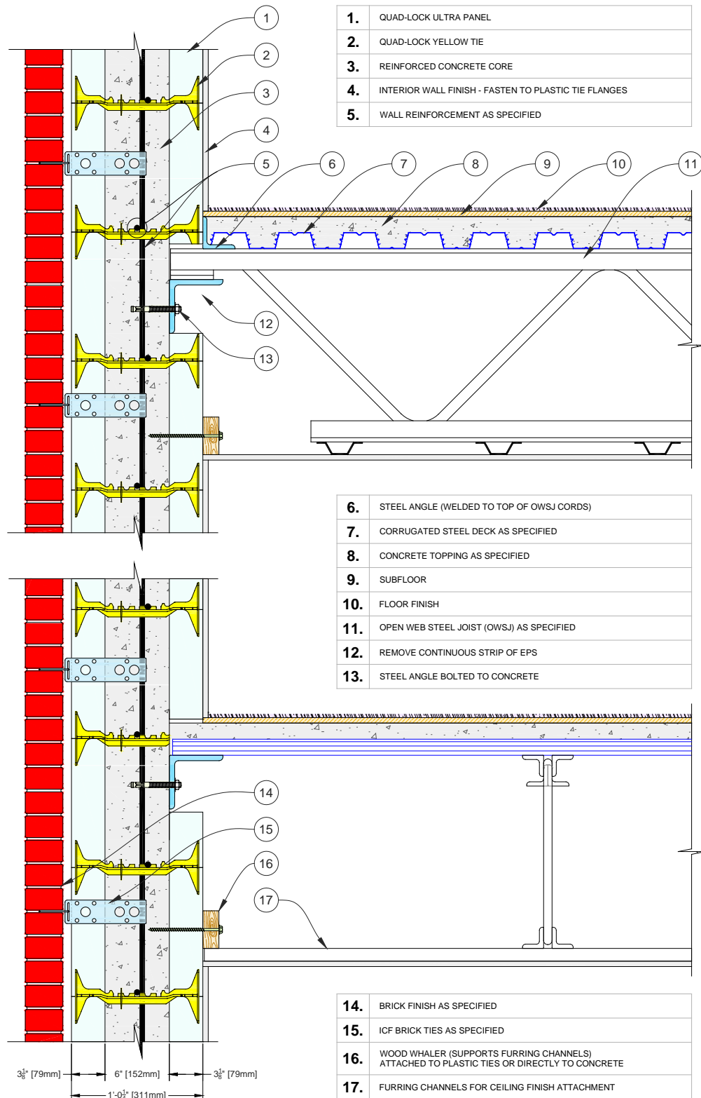
Figure 118: Typical Quad-Lock wall Connection to Composite Concrete and Steel Deck Slab Floor with Steel Joists
