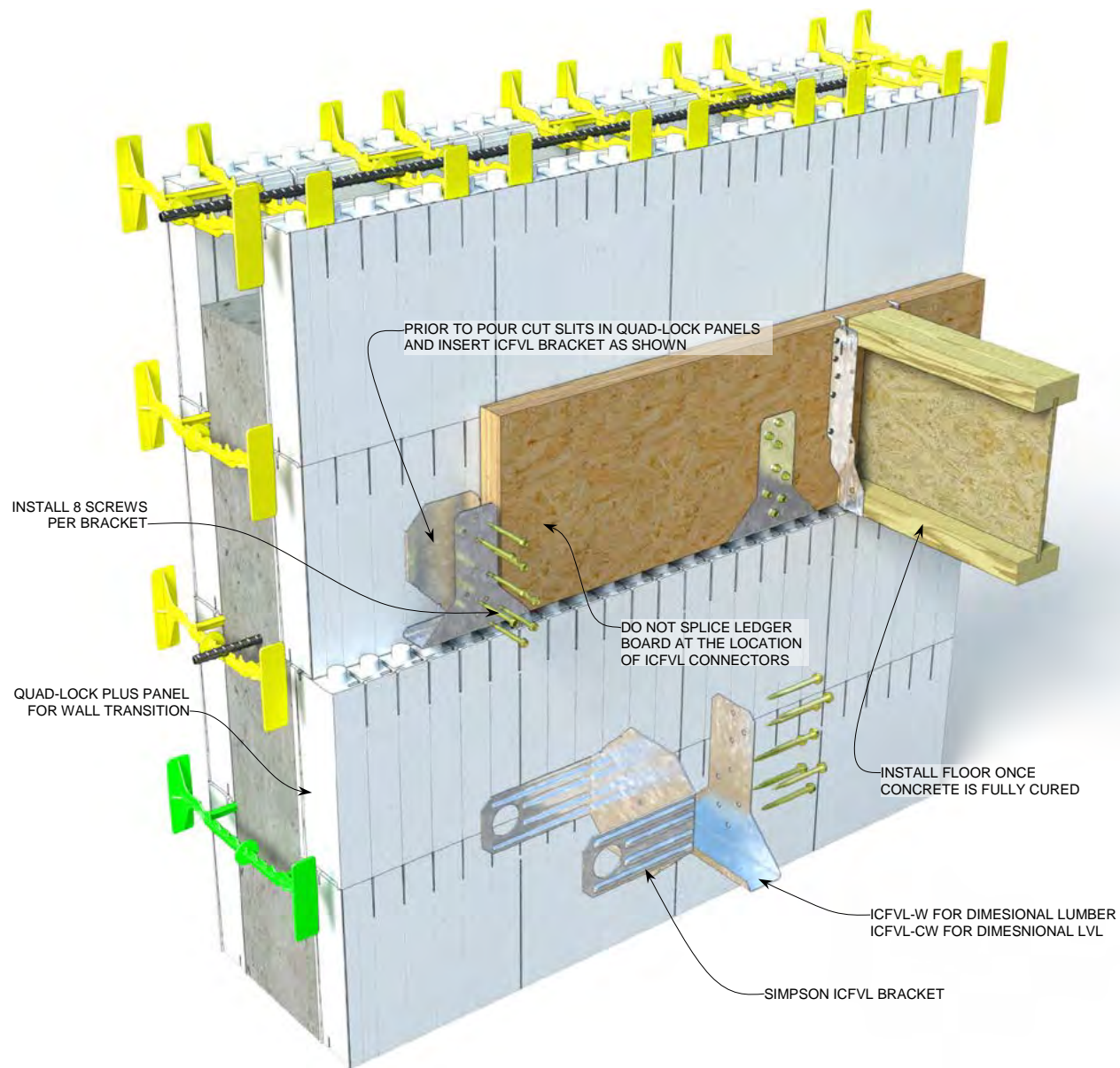
Figure 112: Installation of Floor Ledger with ICFVL Bracket System
