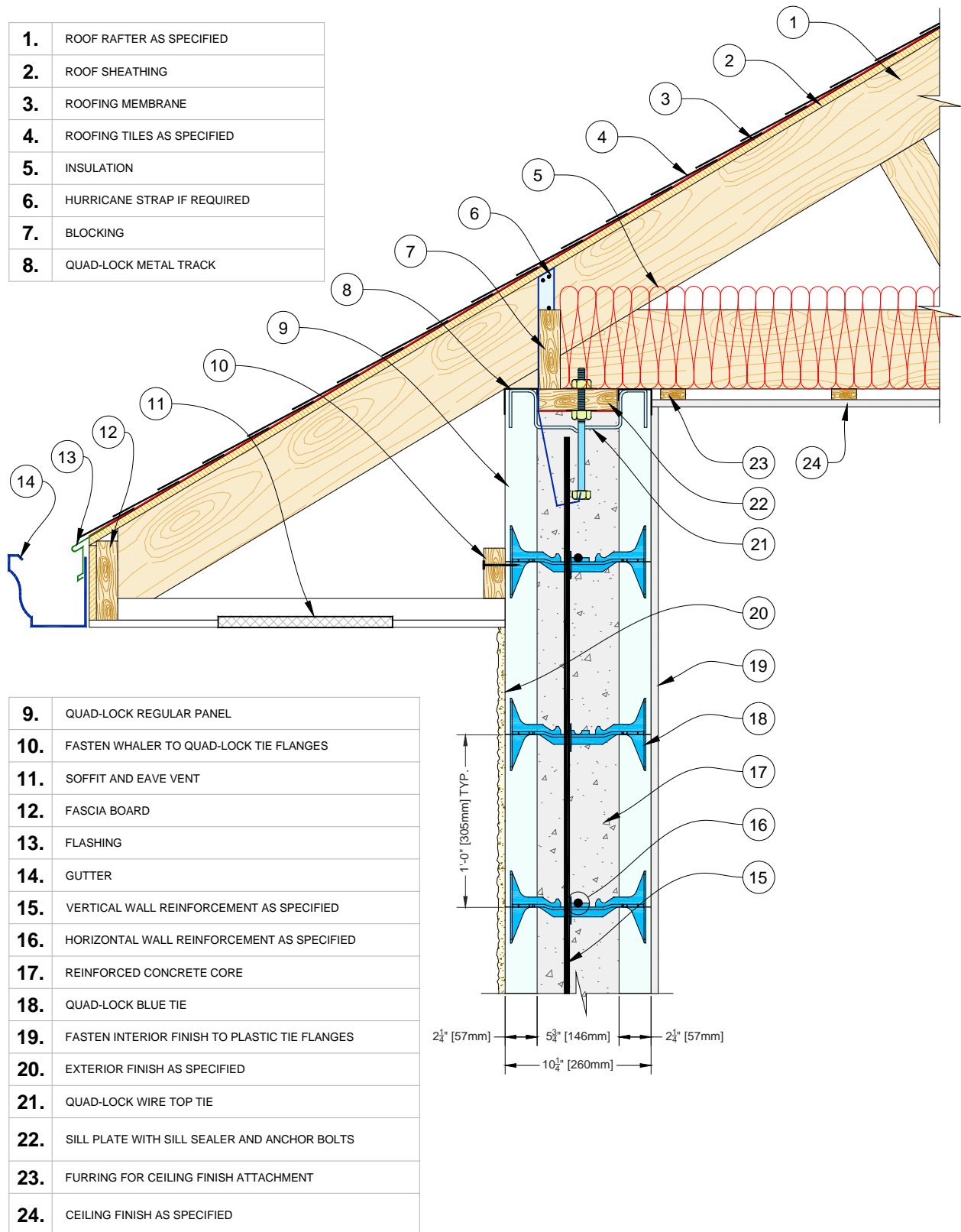
Figure 122: Typical Roof Rafter or Truss - Low Uplift Connection
