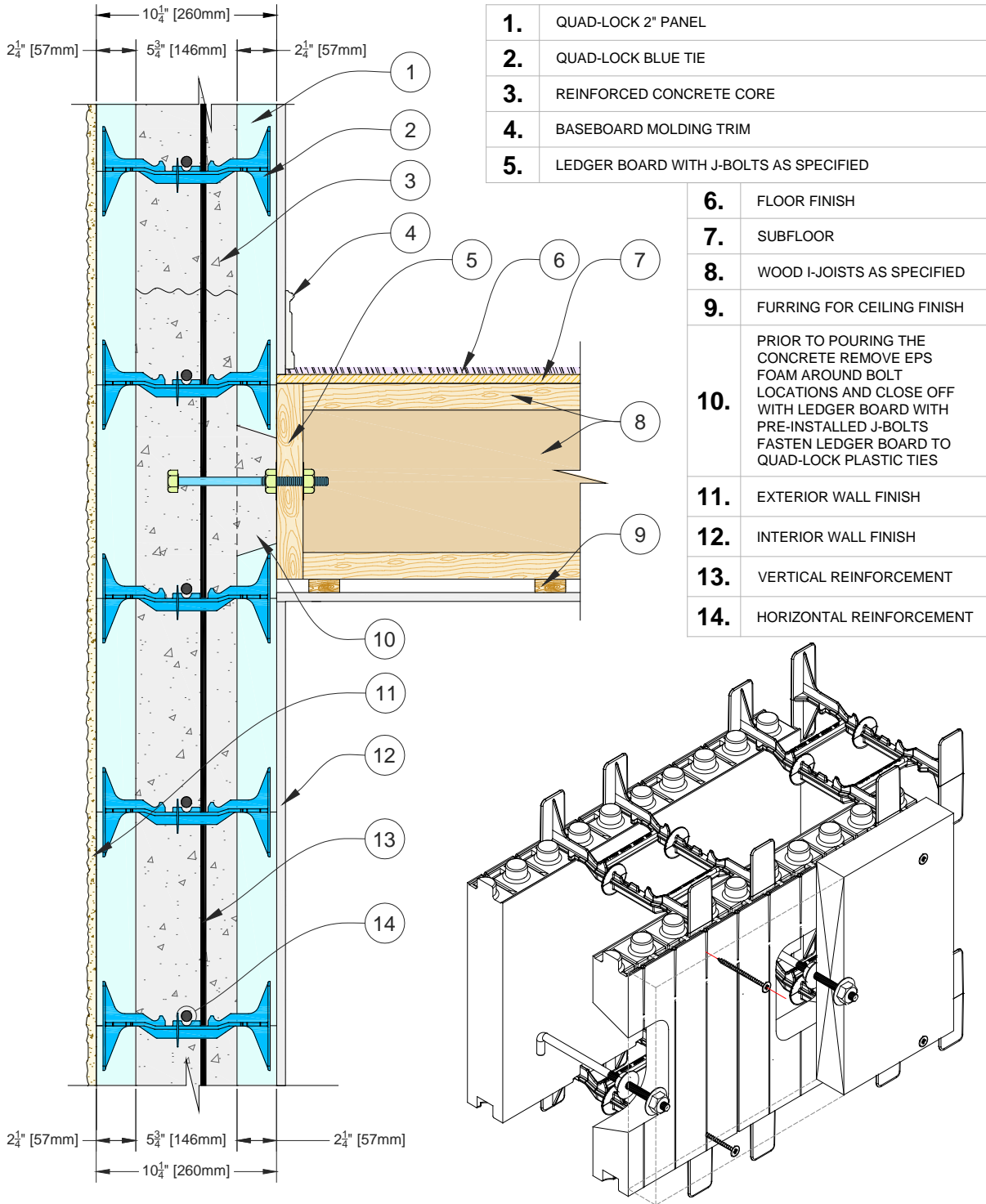
Figure 114: Typical Ledger Board Connection w/ Anchor Bolts
