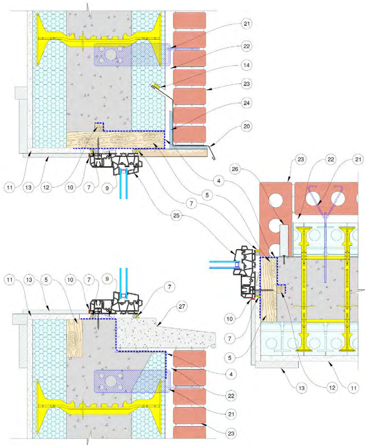
Figure 97: ICF Window Assembly - Wood buck-out, Boxed window centered, Brick veneer
