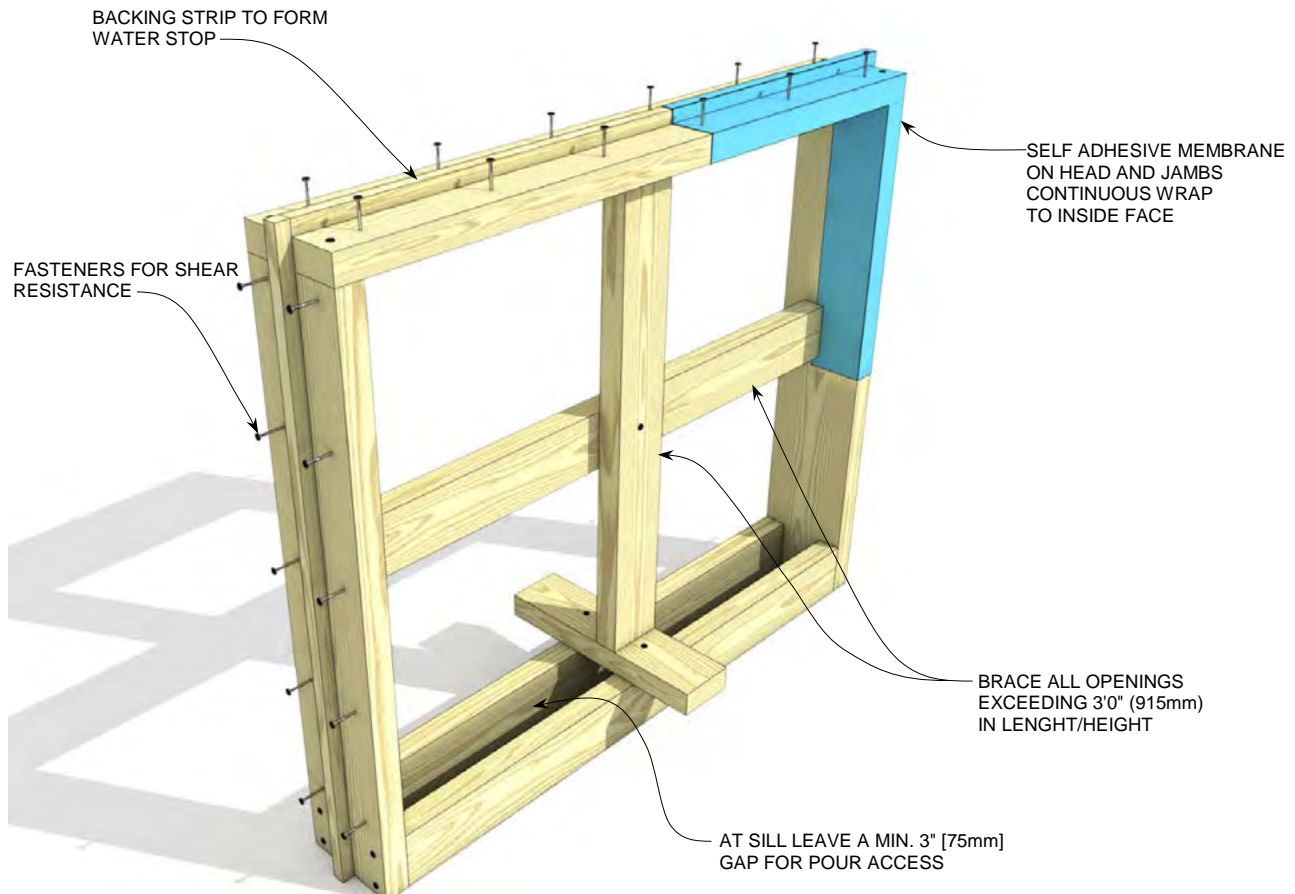
Figure 82: Internal Wood Buck-out with backing strip added to concrete side (lined with Peel & Stick waterproofing membrane)
