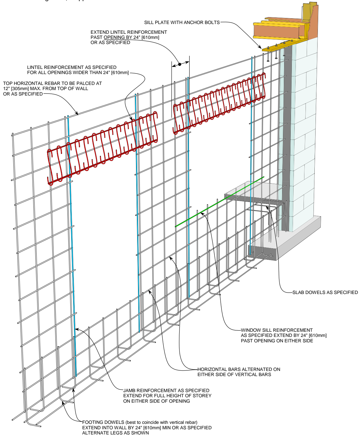
Figure 132: Typical Wall Opening Reinforcement
