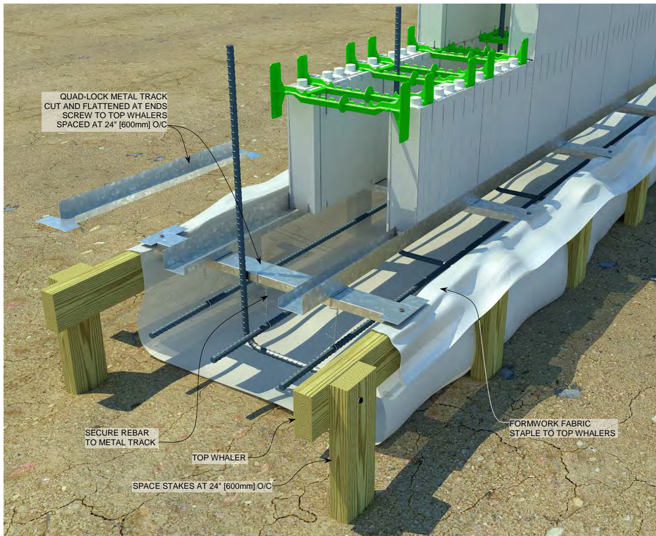
Figure 79: Typical Monolithic Footing / Wall Set Up
