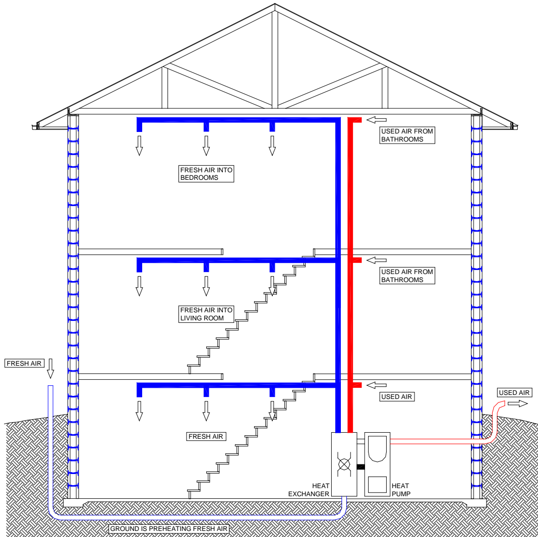
Figure 30: Typical “Passive House” Ventilation System
