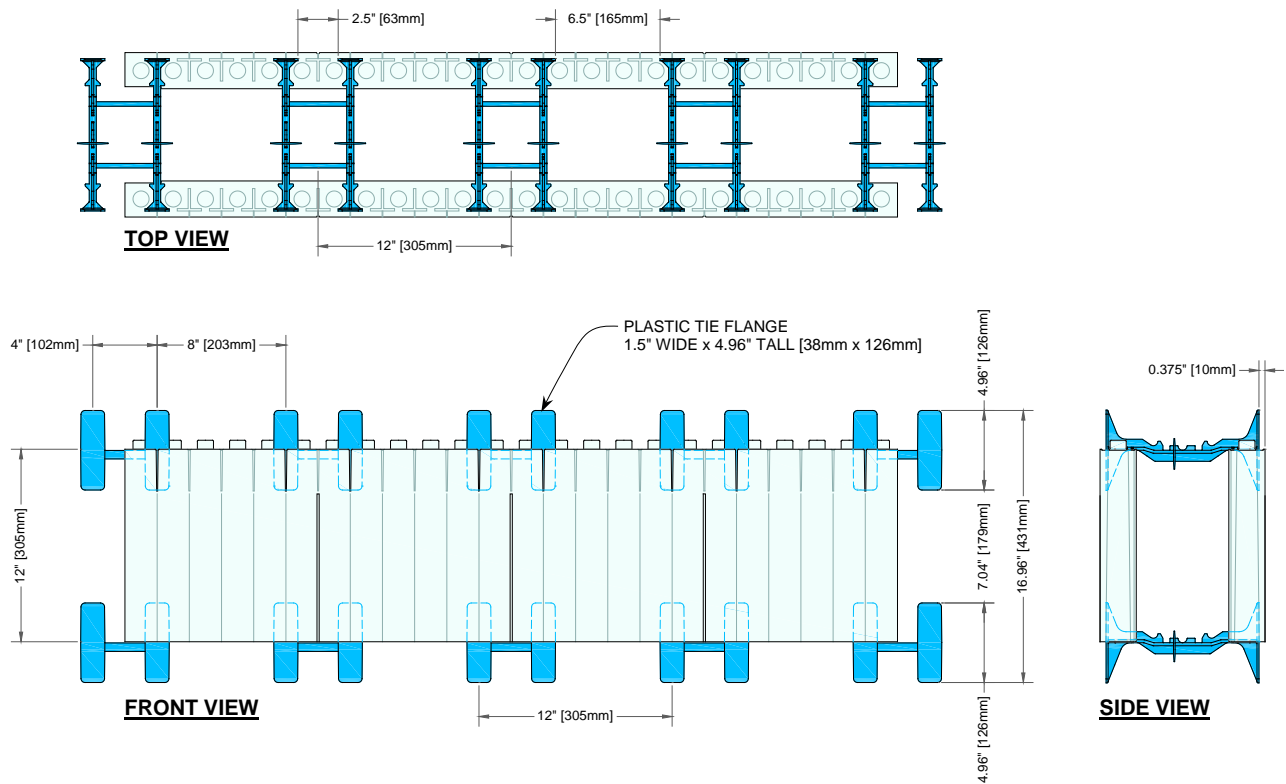
Figure 12: Tie Layout Dimensions
