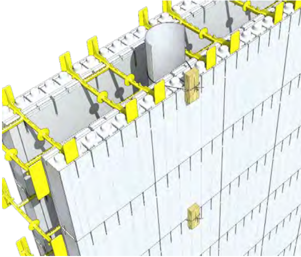
Step 1. Tie Sleeve to Quad-Lock EPS prior to pour.
