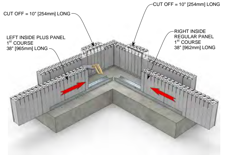
STEP 2 R-38 [U-0.15] 5.75" [146mm] Concrete Wall
