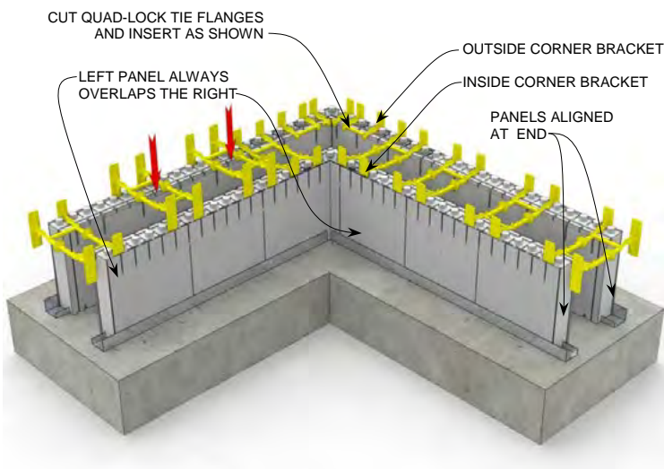
STEP 3 R-28 [U-0.21] 6" [152mm] Concrete Wall
