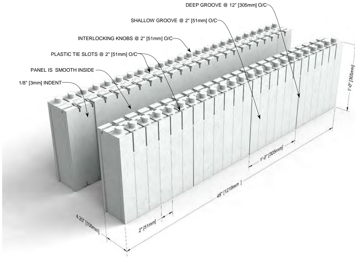
Figure 5: Quad-Lock Plus Panel
