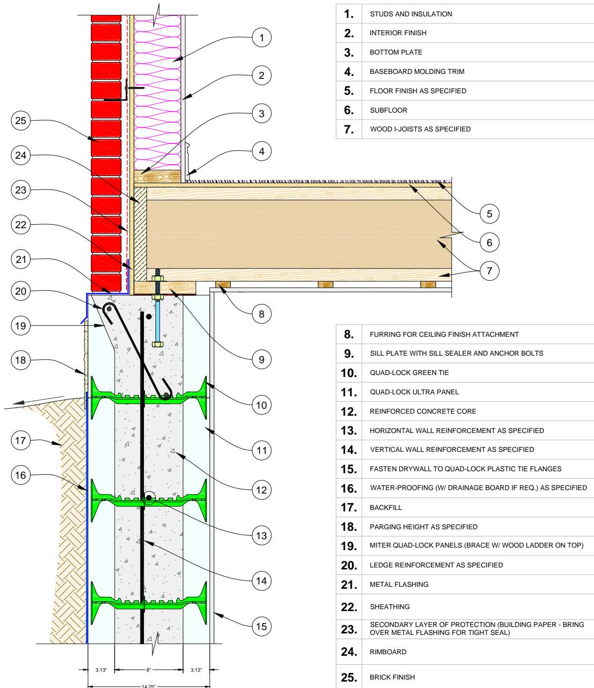
Figure 151: Quad-Lock Wall Tapering out at Top to Provide Support for Brick Finish
