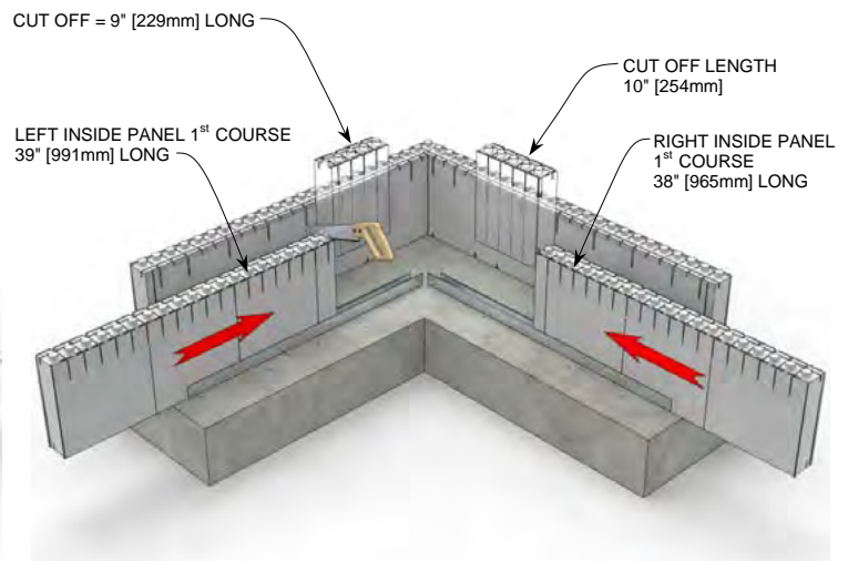
STEP 2 R-28 [U-0.21] 6" [152mm] Concrete Wall
