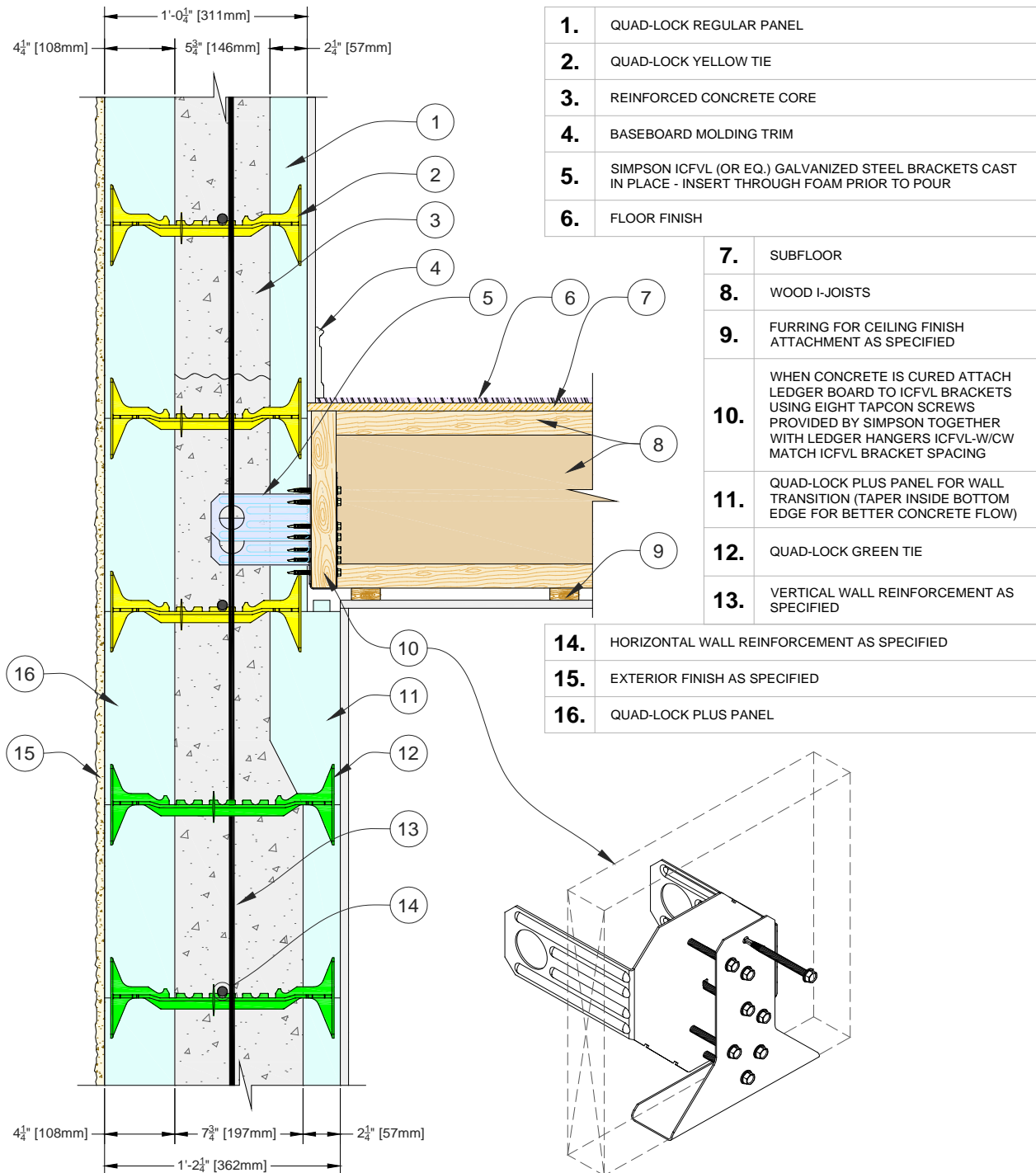
Figure 113: Ledger Installation using ICF Ledger Connectors
