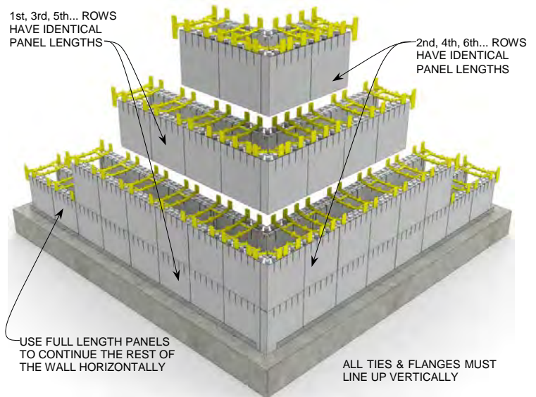
STEP 8 R-28 [U-0.21] 6" [152mm] Concrete Wall
