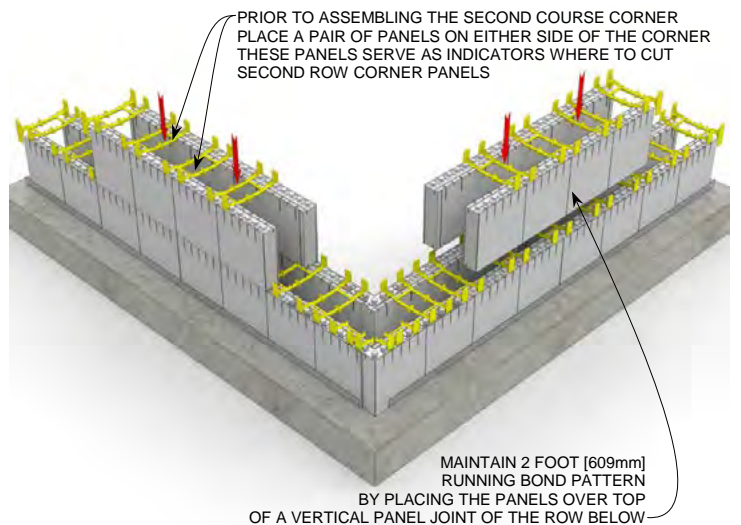
STEP 4 R-28 [U-0.21] 6" [152mm] Concrete Wall (Alternate Method)
