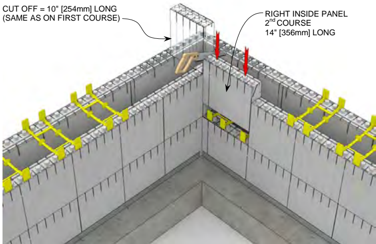
STEP 7 R-28 [U-0.21] 6" [152mm] Concrete Wall (Alternate Method)
