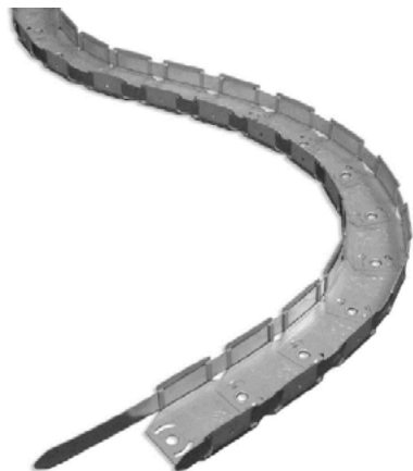
Figure 26: Radius U-Track for Regular Panels
