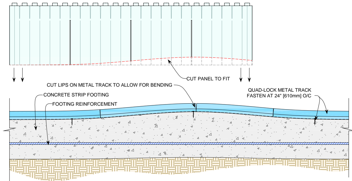
Figure 34: Adapting panels to inconsistencies in footing elevation
