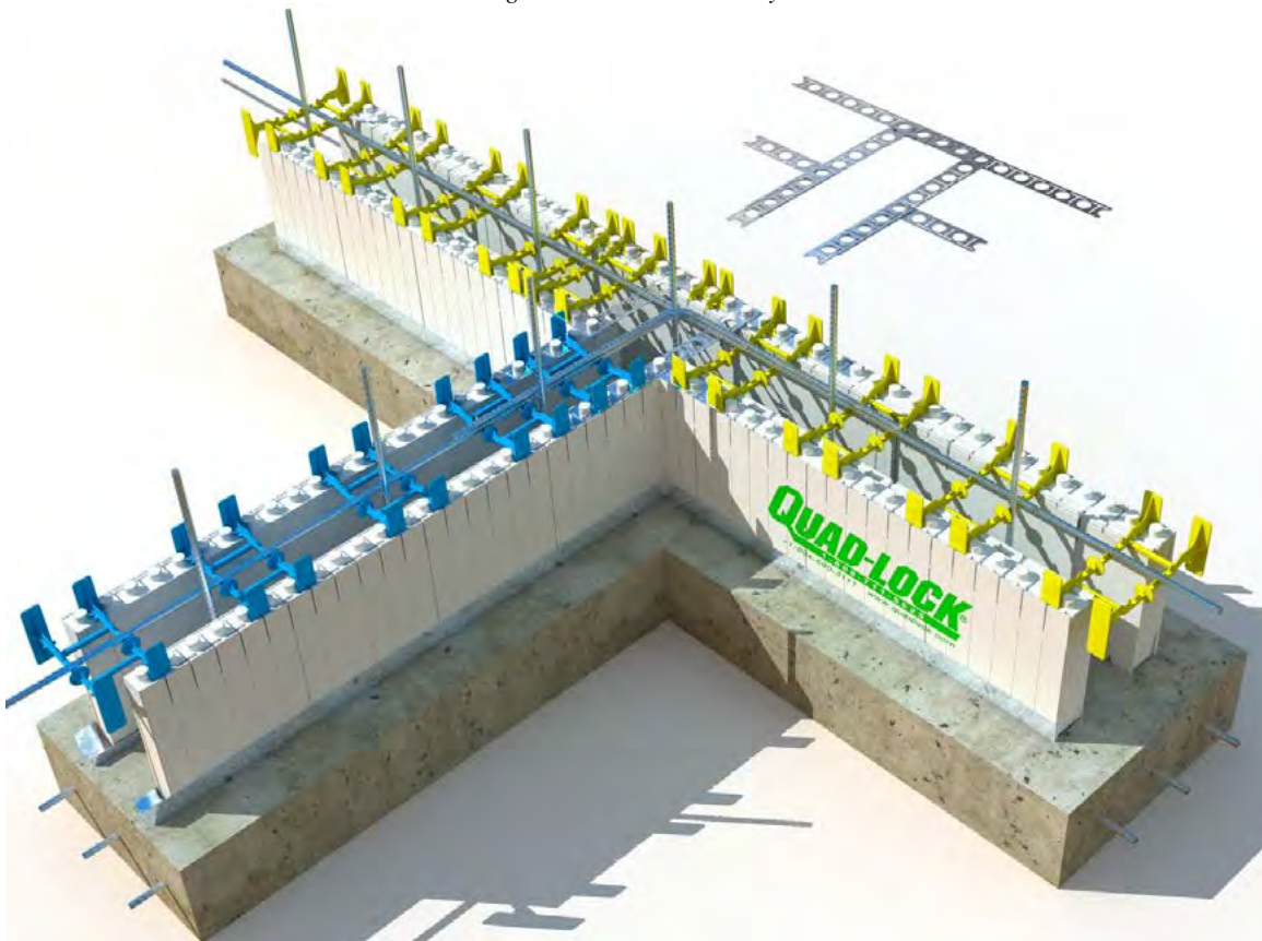
Figure 55: T-Wall Assembly with 2 Outside Corner Brackets and 2 Inside Corner Brackets (3D)
