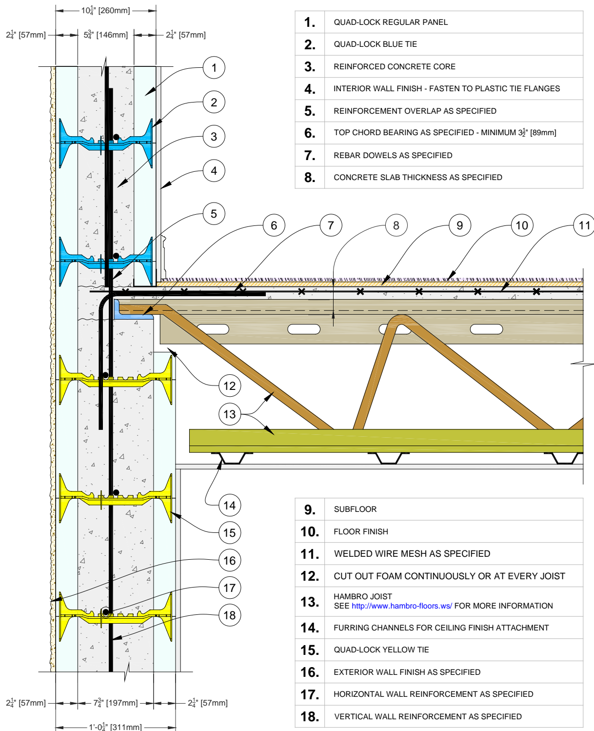
Figure 119: Typical Hambro Composite Floor System Connection
