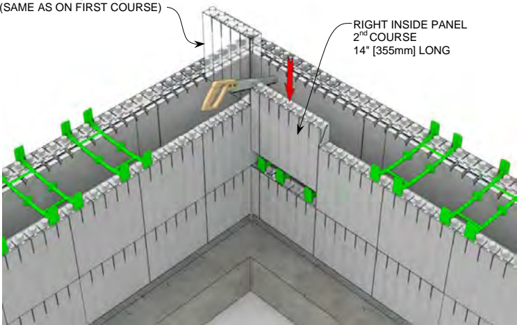
STEP 7 R-30 [U-0.20] 7.75" [197mm] Concrete Wall
