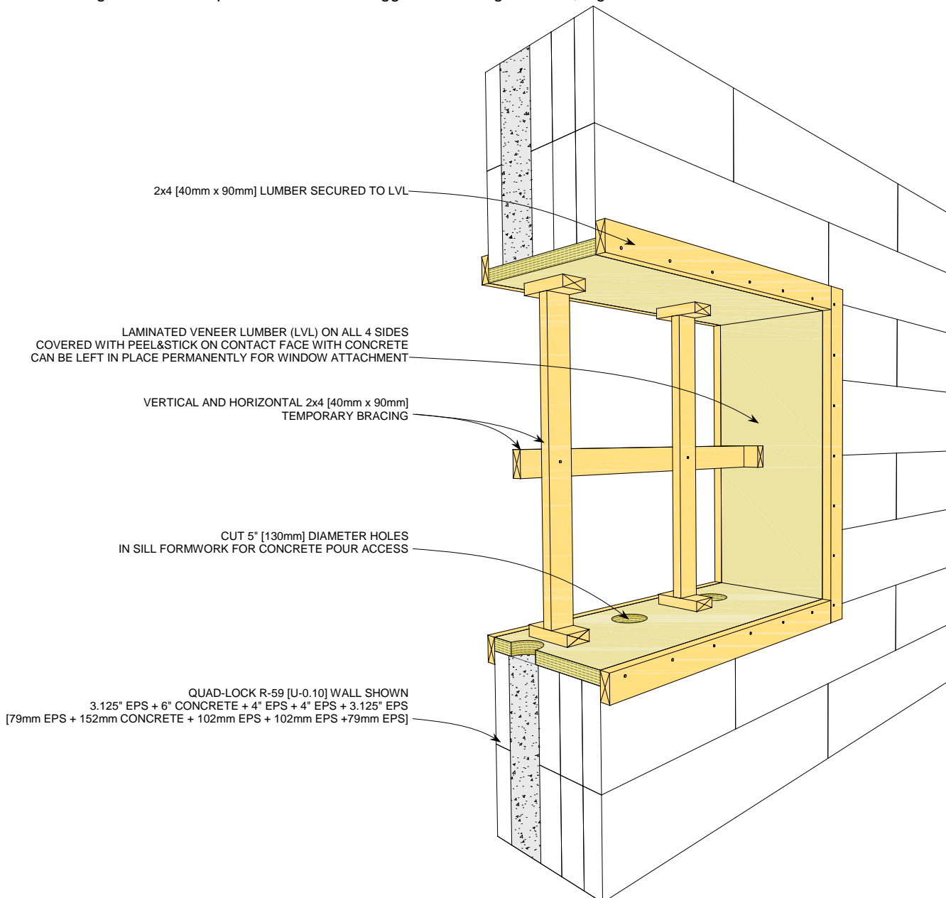
Figure 100: Forming an Opening on Quad-Lock R-59 [U-0.10] Wall
