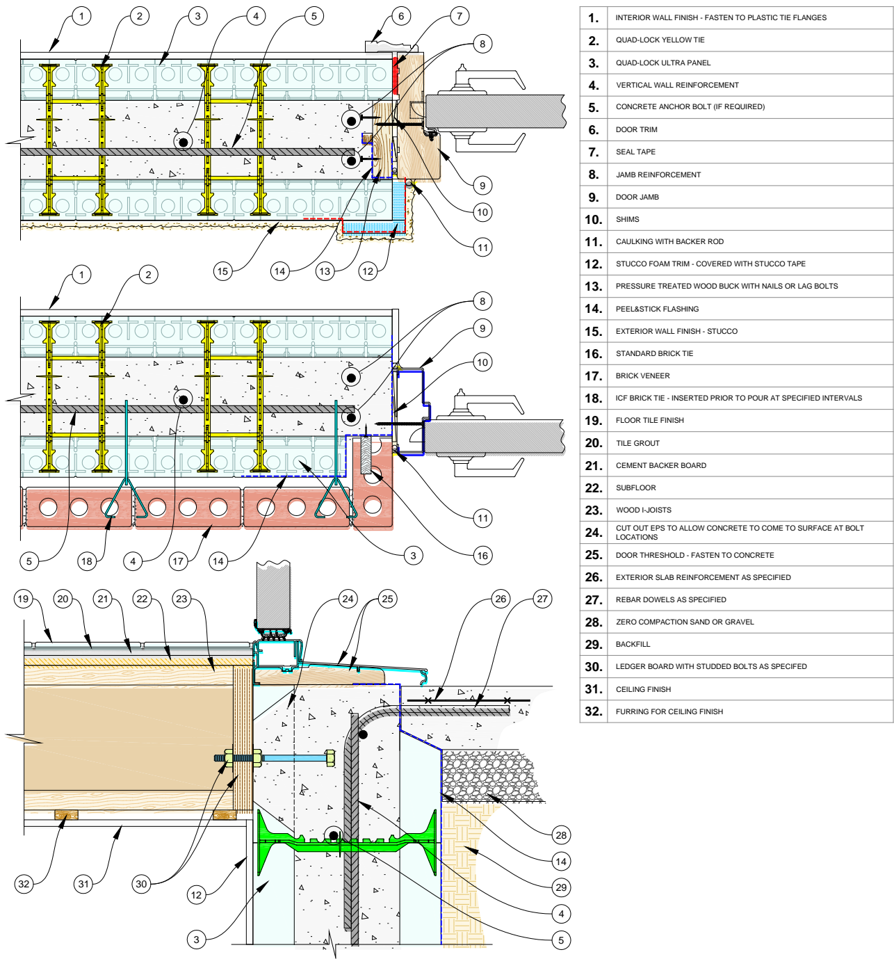
Figure 103: Exterior Door at Jamb(Residential and Commercial) and Threshold
