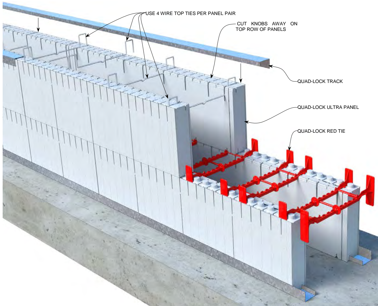
Figure 51: Finishing the Top of Walls with Metal Tracks and Wire Top Ties
