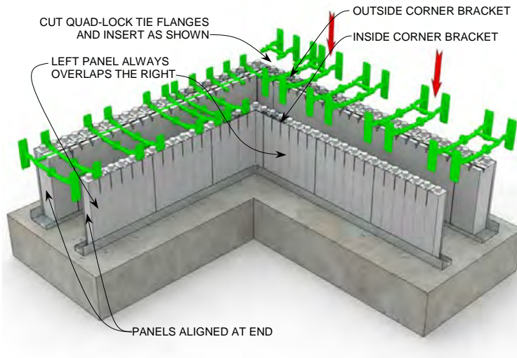
STEP 3 R-30 [U-0.20] 7.75" [197mm] Concrete Wall
