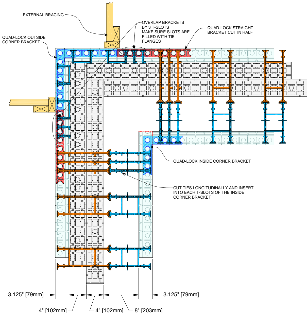
Figure 65: Extender Tie Assembly for Corners
