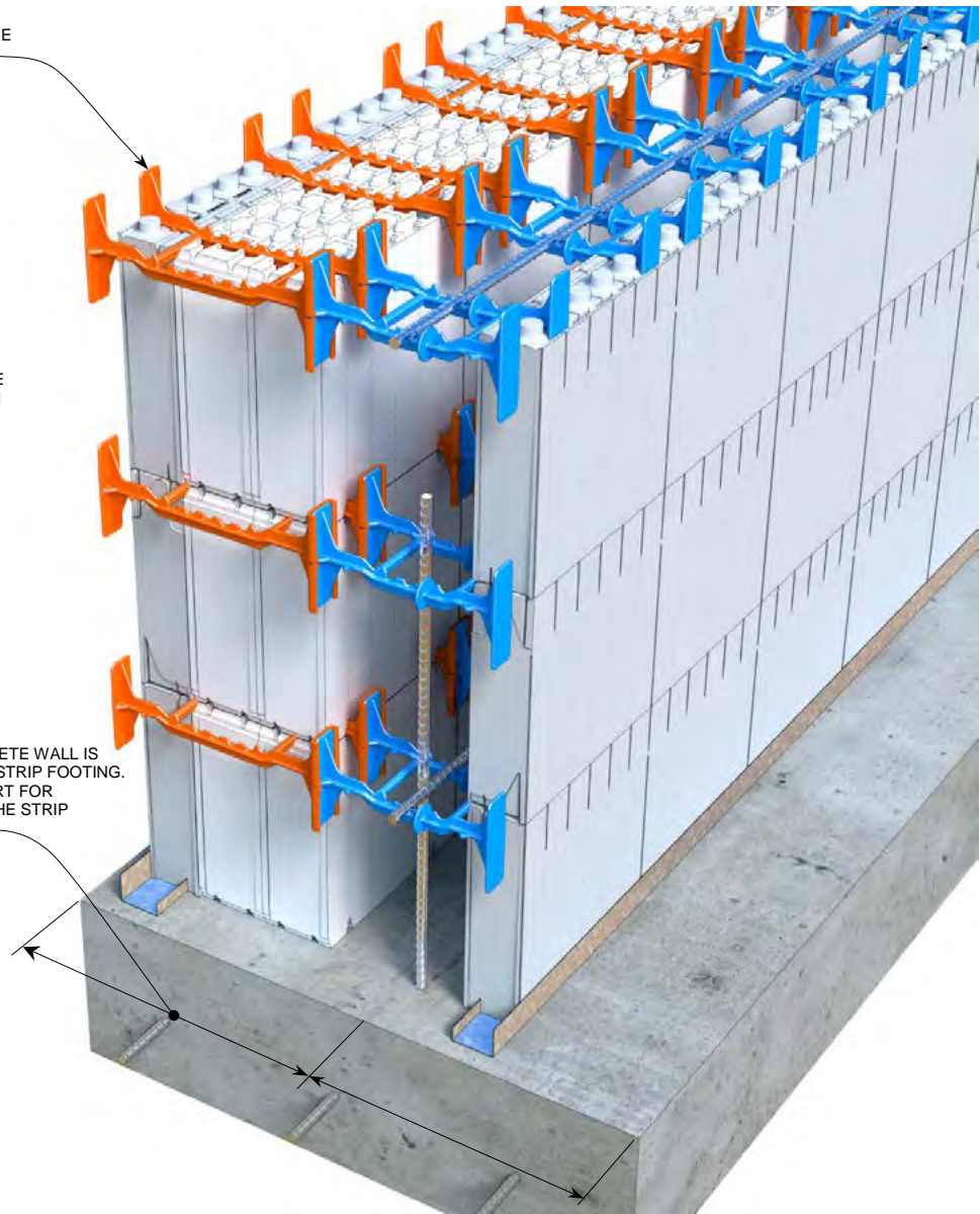
Figure 66: Extender Tie Assembly (20" [508mm] cavity shown)
