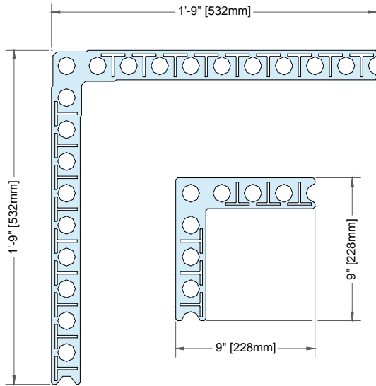
Figure 17: Inside and Outside Corner Brackets
