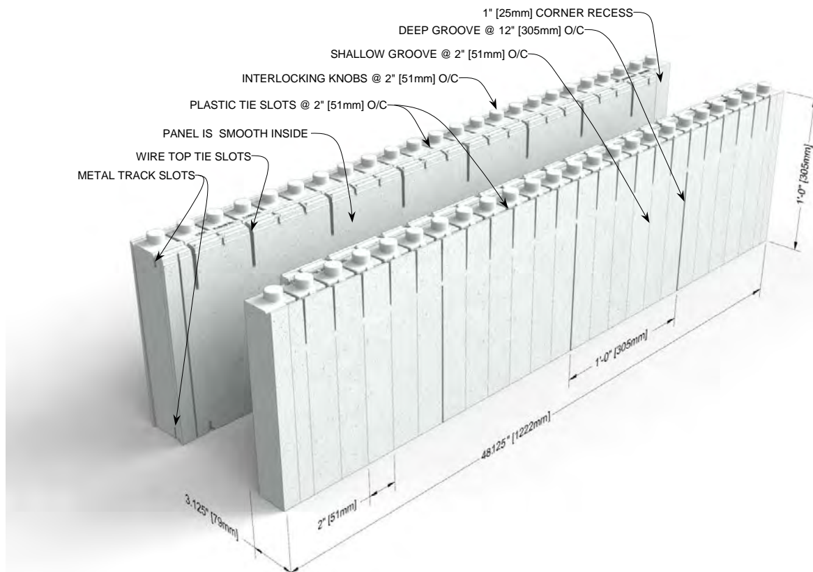
Figure 4: Quad-Lock Ultra Corner Panels
