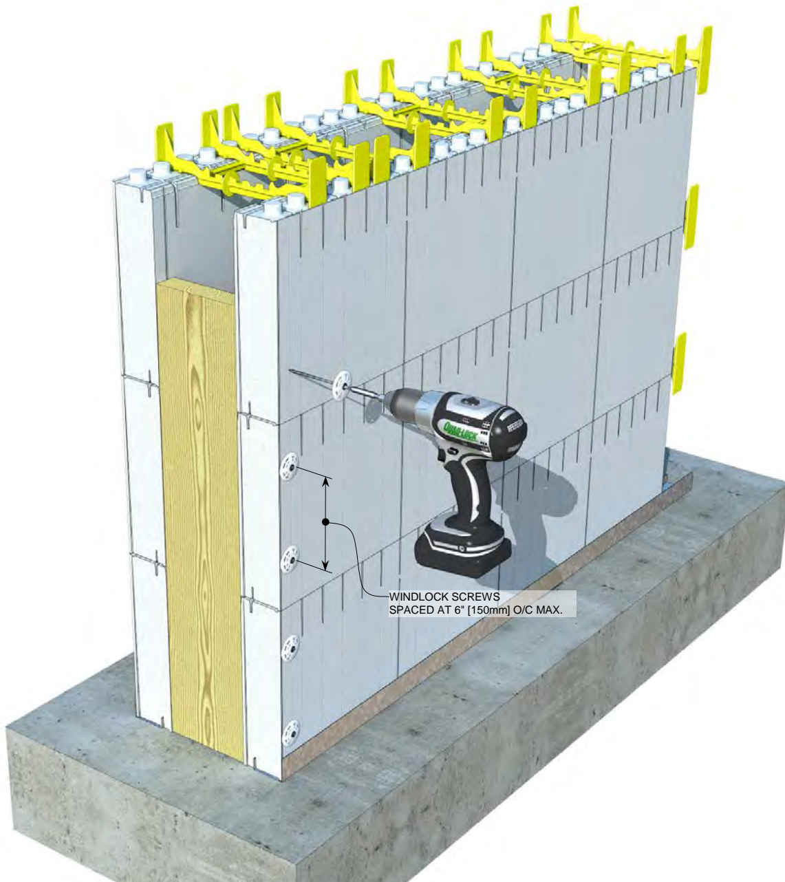
Figure 57: Bulkhead Formed with Lumber and Windlocks
