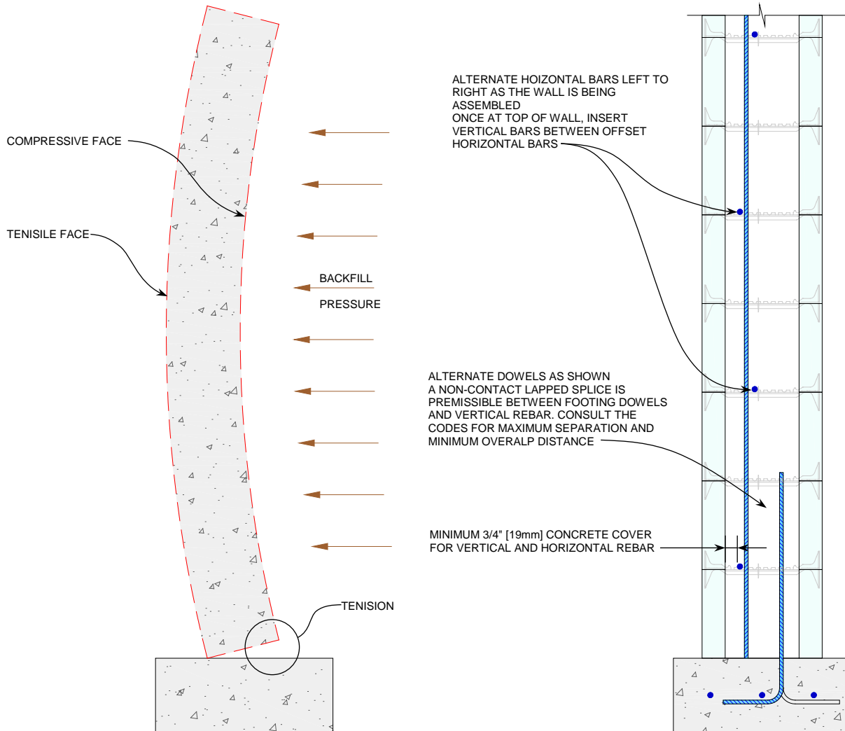
Figure 127: Position of Reinforcement within Quad-Lock Walls
