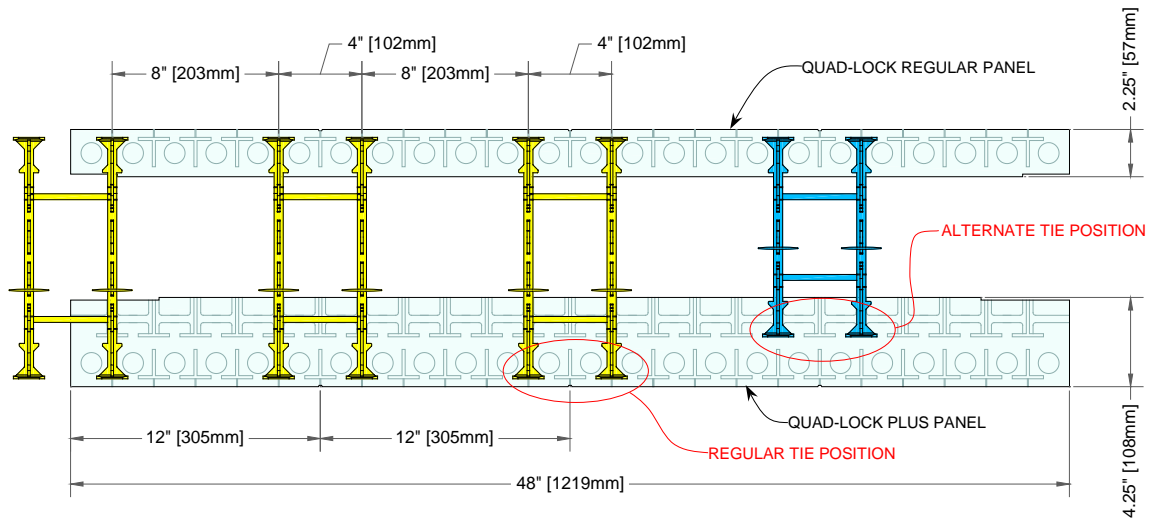
Figure 11: Quad-Lock Plus Panel - Positioning of Ties
