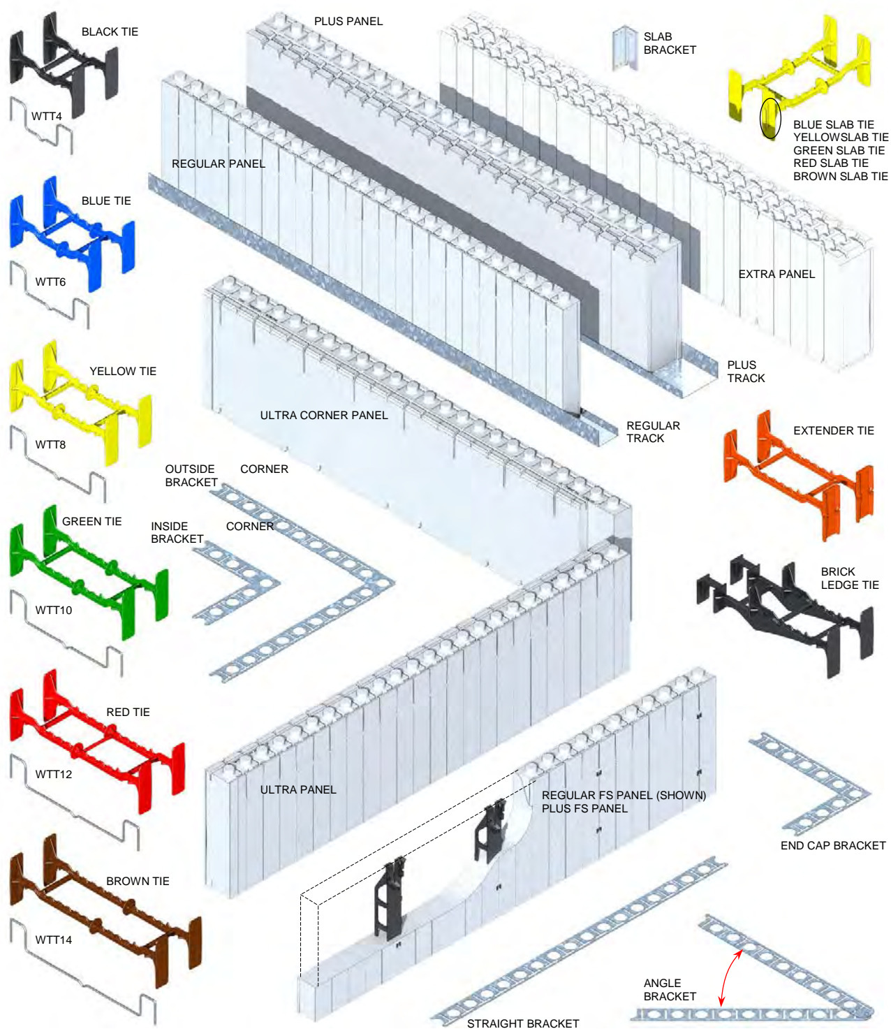
Figure 1: Quad-Lock Components
