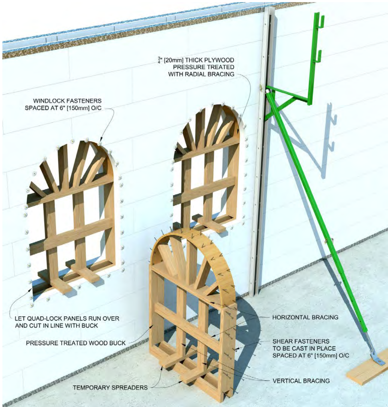
Figure 99: Arched Openings
