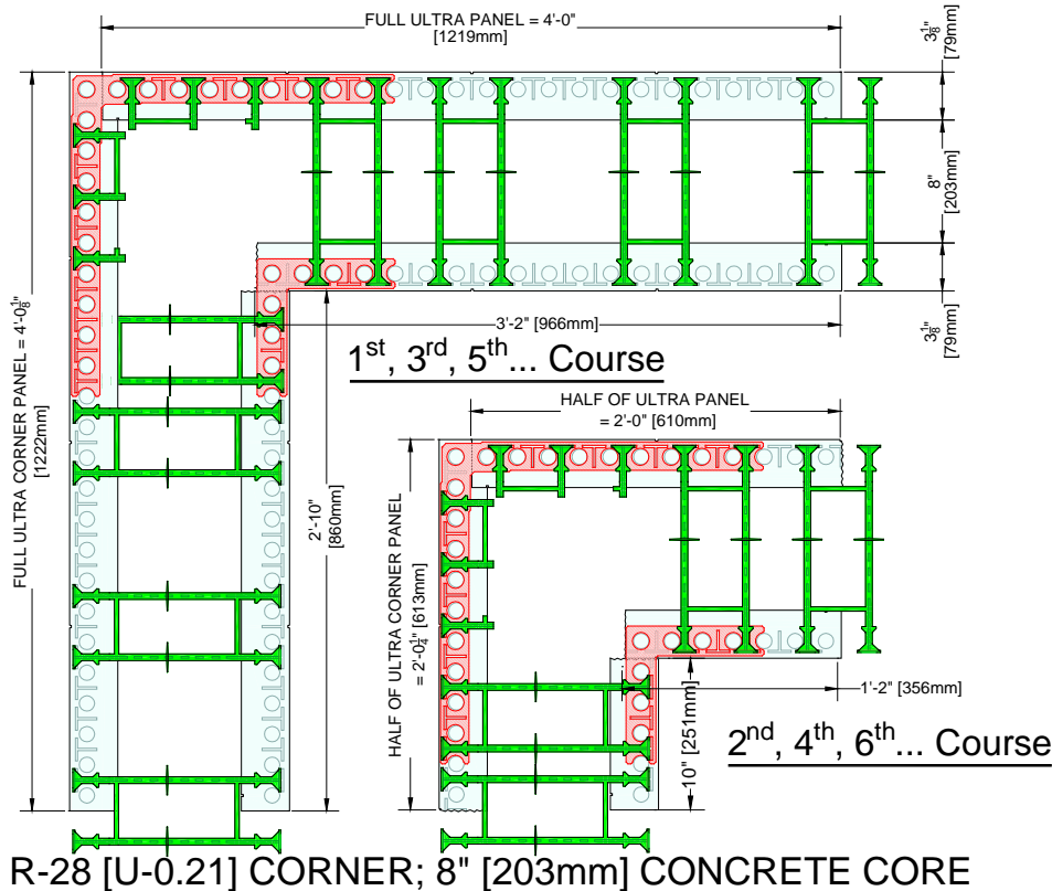
Figure 49: Panel/Tie Combination for R-28 [U-0.21] 8" Concrete Cavity
