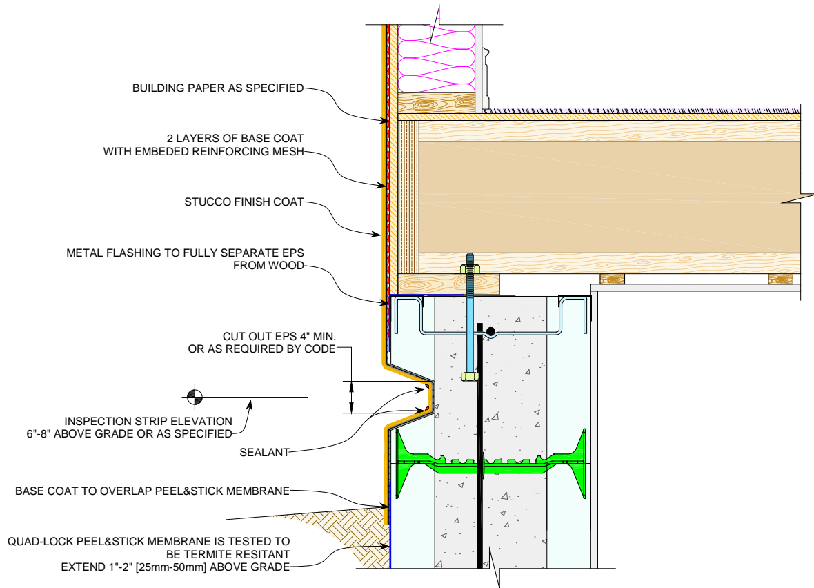
Figure 77: Termite Protection for Foundation Walls
