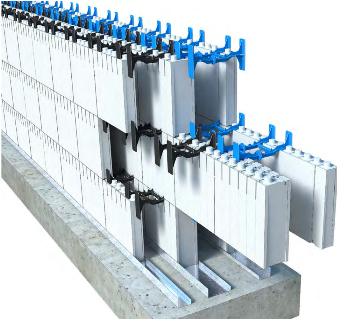
Figure 75: Double Wall / Common Wall
