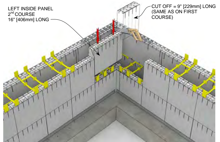
STEP 6 R-28 [U-0.21] 6" [152mm] Concrete Wall (Alternate Method)
