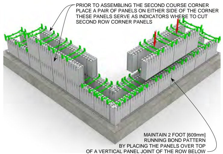
STEP 4 R-38 [U-0.15] 5.75" [146mm] Concrete Wall
