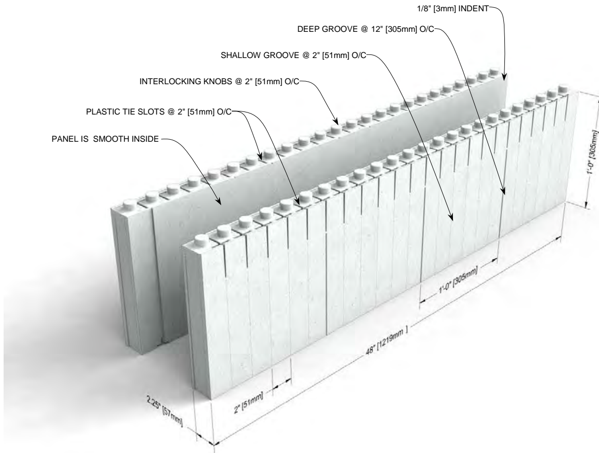
Figure 2: Quad-Lock Regular Panels
