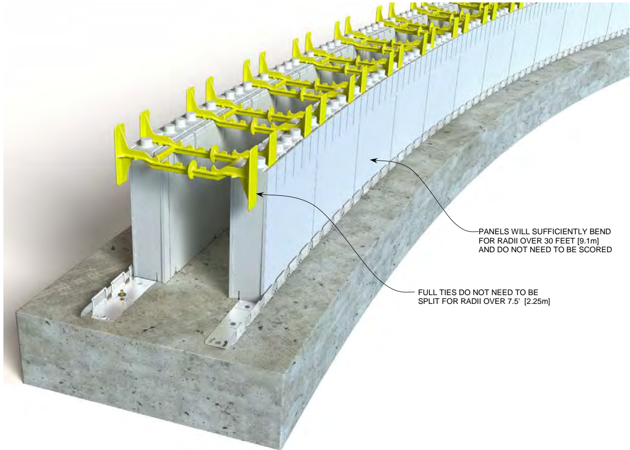
Figure 62: Radius Wall (wide radius)
