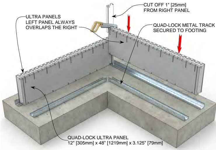
STEP 1 R-28 [U-0.21] 6" [152mm] Concrete Wall (Alternate Method)
