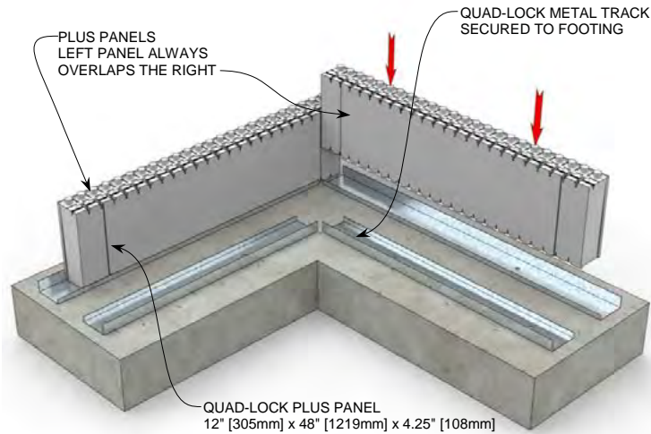
STEP 1 R-38 [U-0.15] 5.75" [146mm] Concrete Wall
