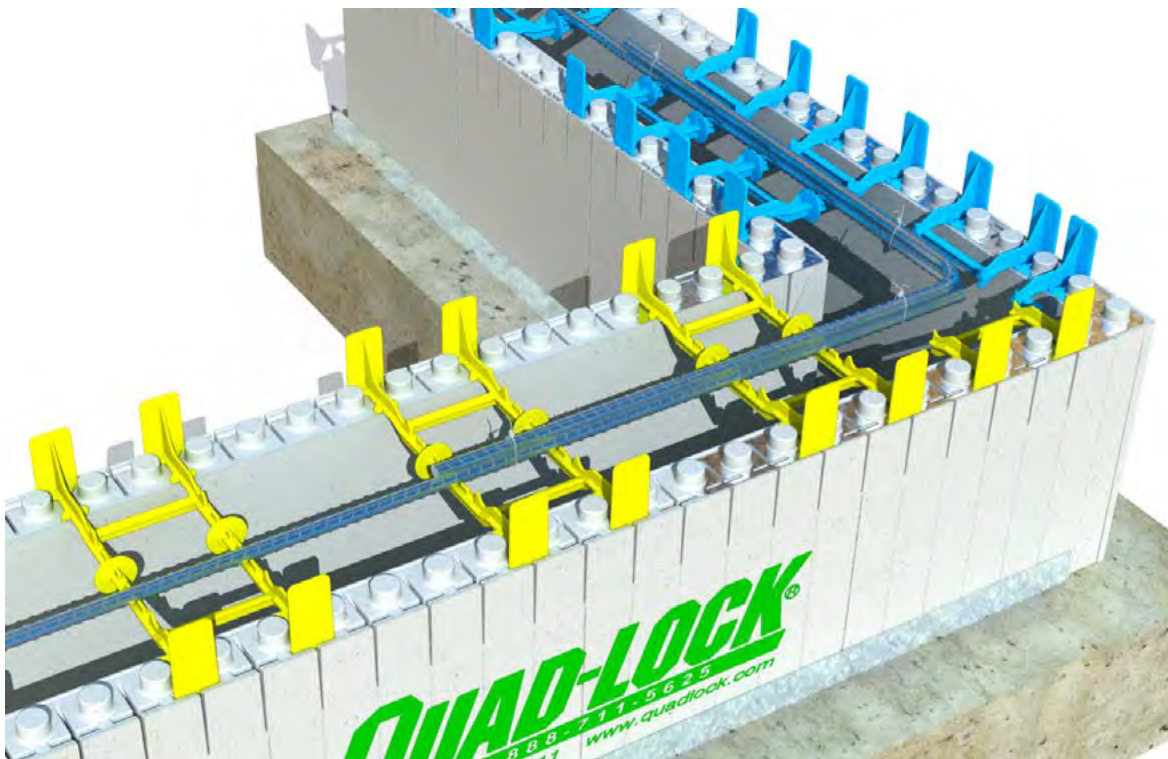
Figure 129: Sample Rebar Placement at Corners & T-Walls
