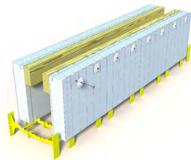
Double 2x4 [50mm x 100mm] secured with Wind-Locks
