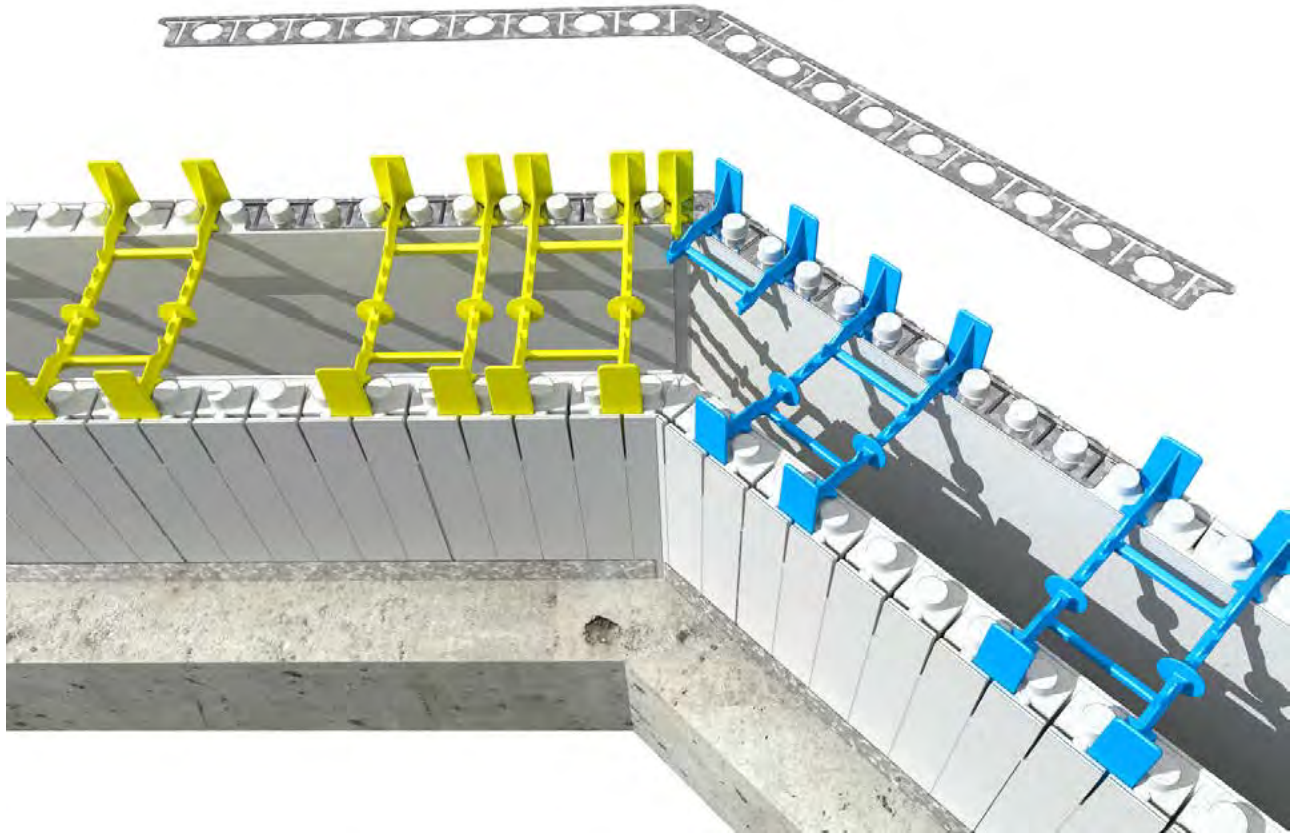
Figure 59: Assembly of Angles
