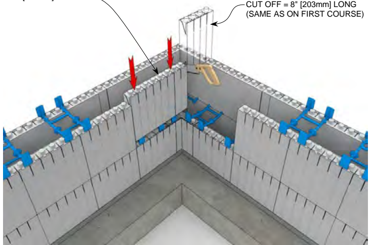
STEP 6 R-22 [U-0.28] 5.75" [146mm] Concrete Wall
