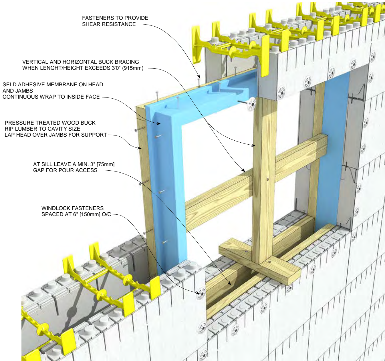
Figure 84: Internal buck-out with water-stop flashing, bracing, and ICF panels fastened to wood members
