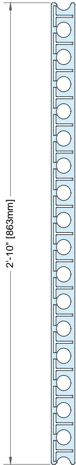
Figure 23: Straight Bracket
