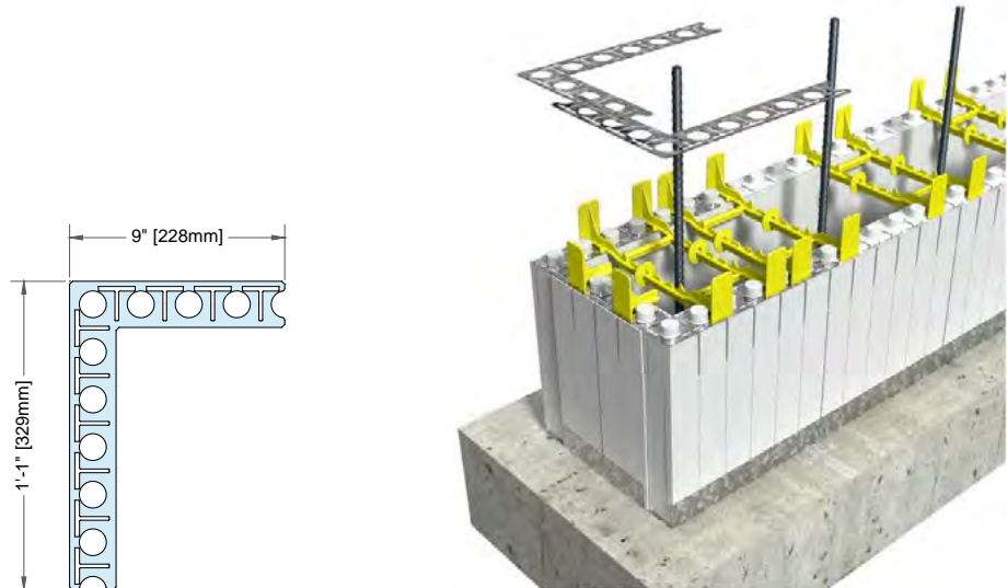
Figure 21: End Cap Bracket
