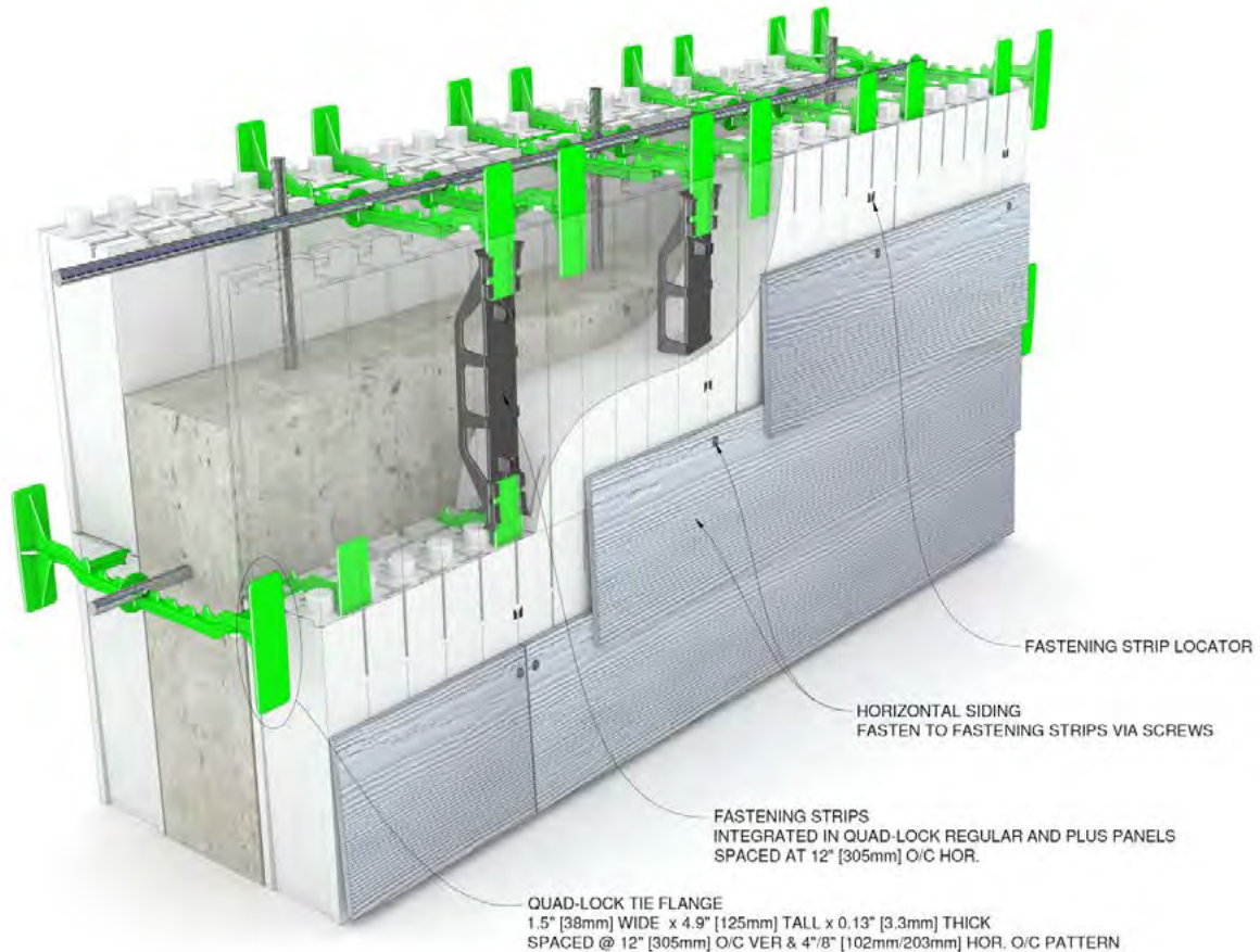
Figure 139: Cladding Details
