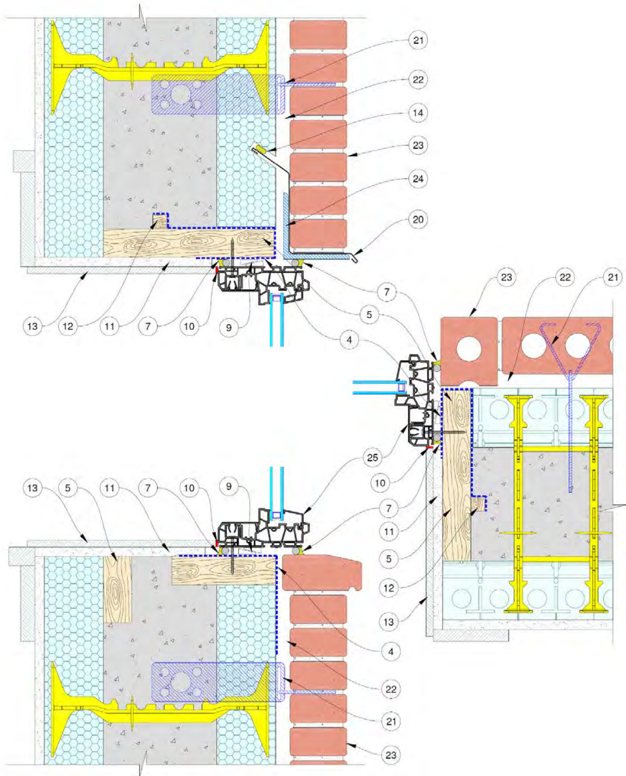
Figure 91: ICF Window Assembly - Wood buck-out, Boxed window flush, Brick veneer
